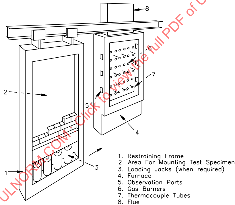
Figure 3.2 Test furnace
