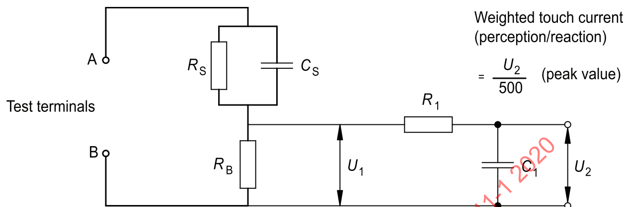
Figure C.3 Circuit of the leakage current meter
