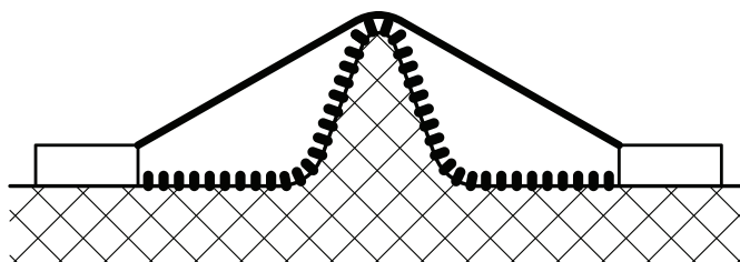
Figure A.2 Clearance gap for rib and uncemented joint with groove
