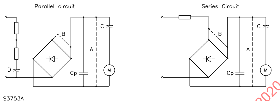
Figure B.1 Simulation of fault conditions
