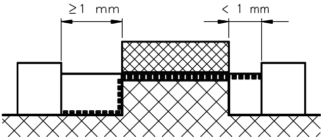
Figure A.3 Clearance gap for uncemented joint and diverging-sided groove
