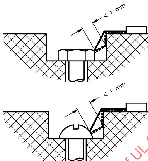
Figure A.4 Clearance gap between wall and screw
