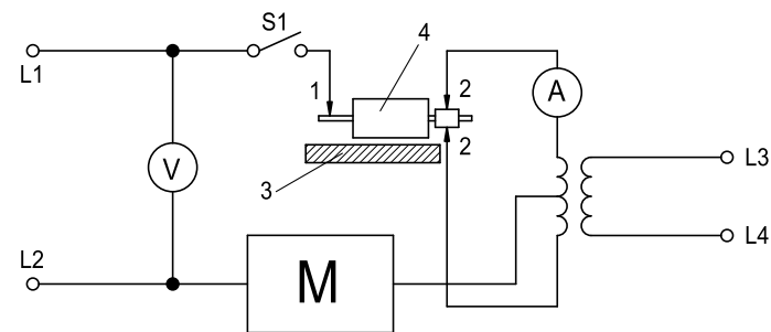
Figure 3 Overload test of a class II armature
