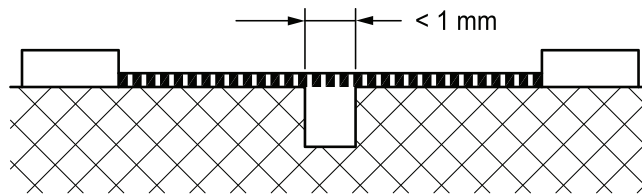
Figure A.1 Clearance gap for parallel sided and V-shaped groove
