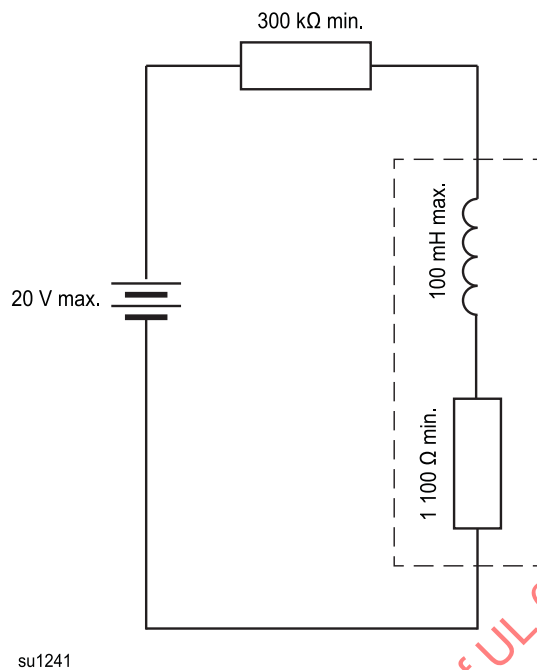
Figure A.7 – Simple inductive circuit
