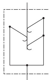
Figure 5b - Example of three connecting elements which are not independent
