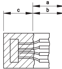
Figure 4a - Partially coated board
