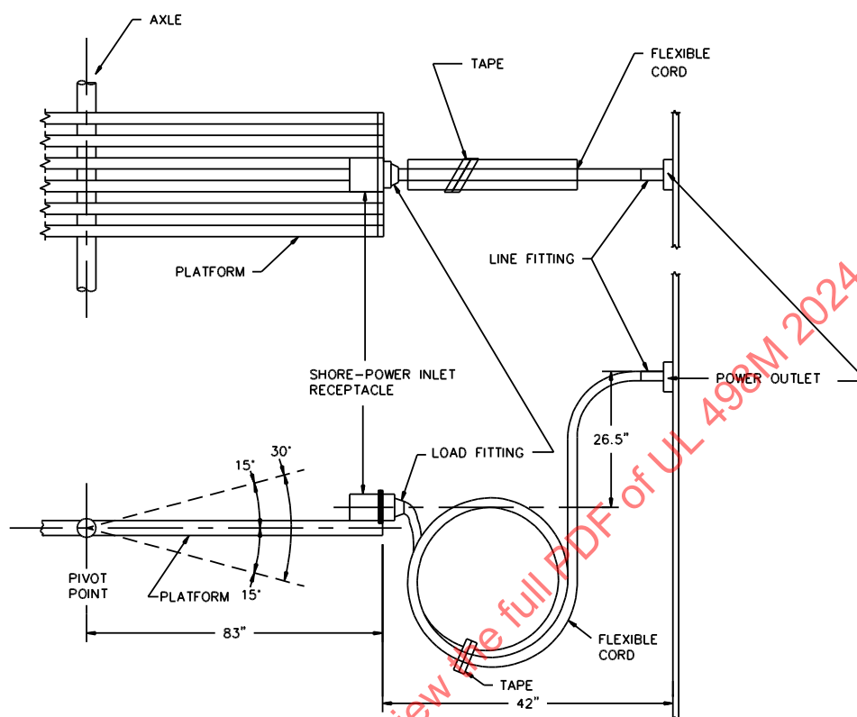
Figure 12.1 Mechanical Strength Test Apparatus
