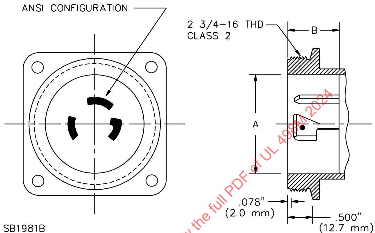
Figure 6.1 Dimensions of a Shore Power Inlet
