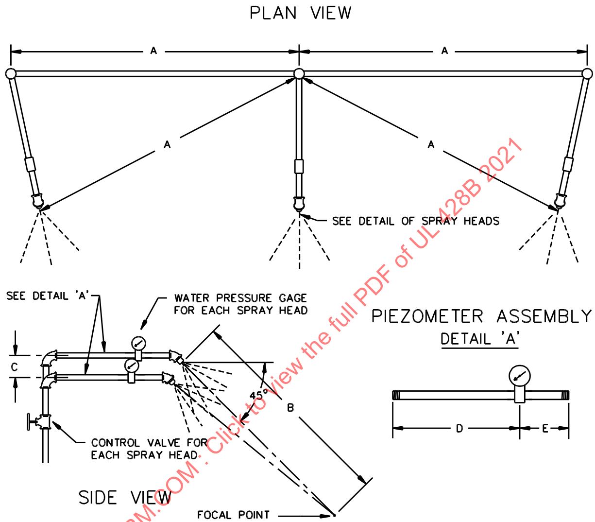
Figure 38.1 Rain-test spray piping
