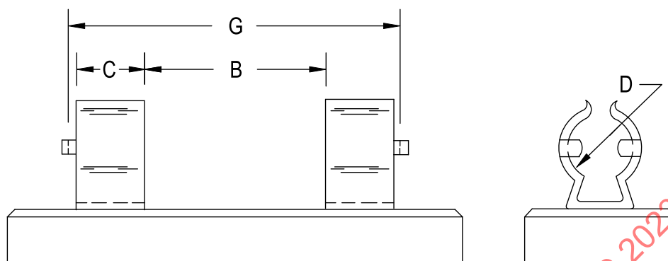
Figure 7.6A Class K fuseholder – Ferrule-contact type
