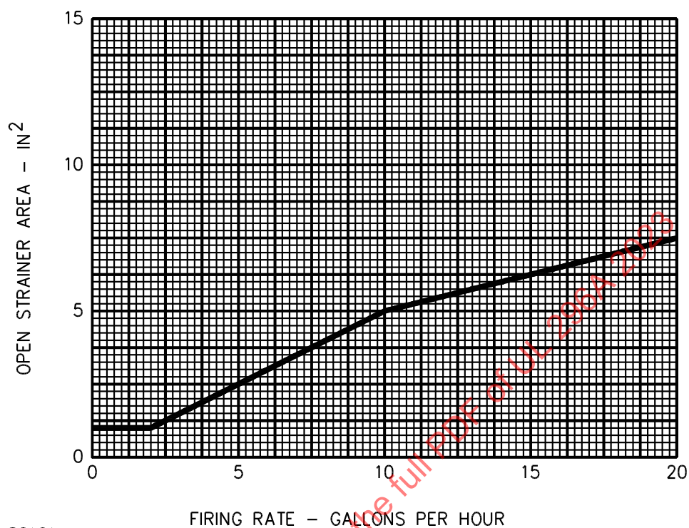
Figure 43.1 Strainer area for No. 1 fuel oil a
