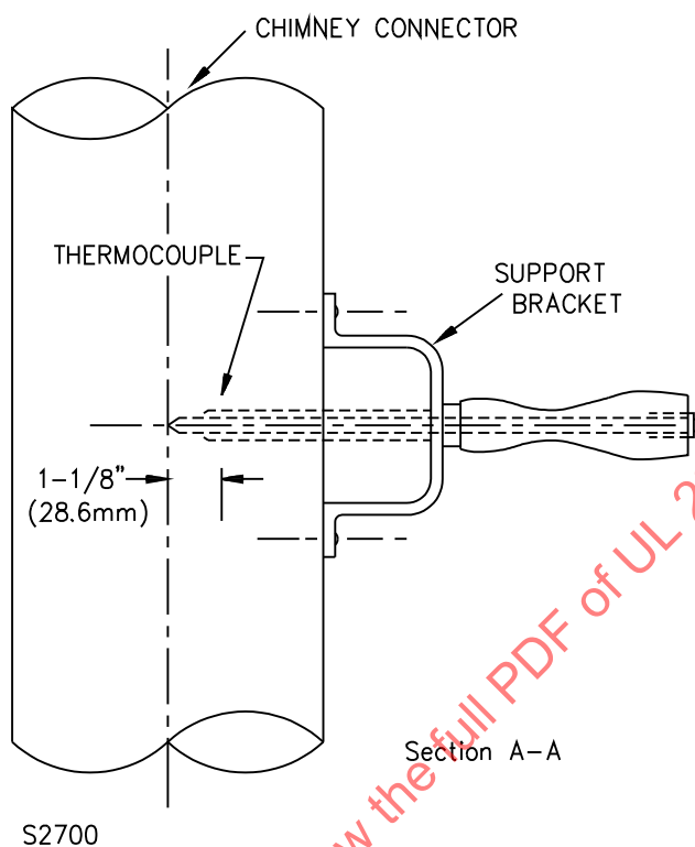
Figure 23.3 Flue gas thermocouple and support bracket
