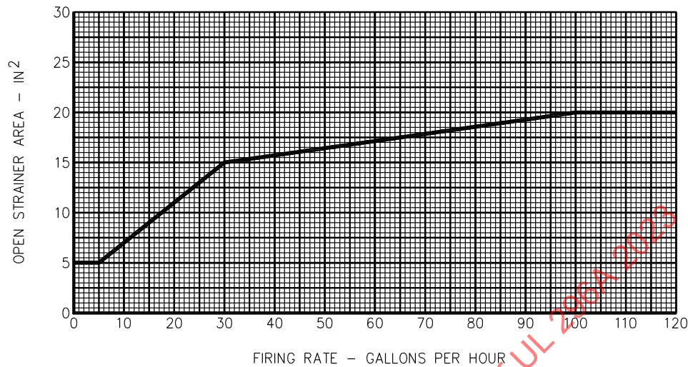
Figure 43.3 Strainer area for Nos. 4, 5, 6 fuel oils a
