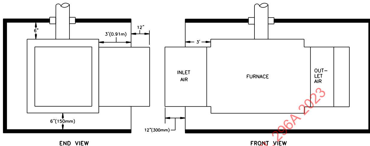
Figure 87.6 Enclosure for horizontal furnace – standard clearances
