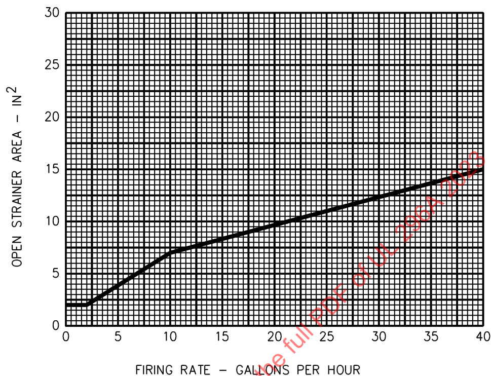
Figure 43.2 Strainer area for No. 2 Fuel oil a
