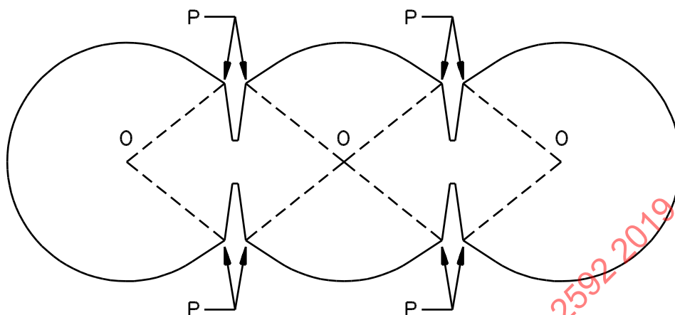
Figure 6.1 Definition of regions of valley slopes on which thickness measurements shall not be made on parallel constructions
