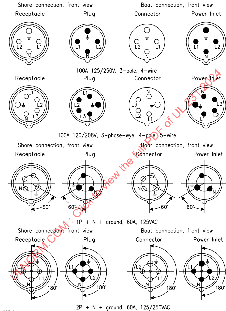
Figure 8.3 Common pin-and-sleeve type configurations
