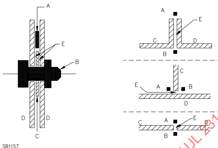
Figure 15.1 Clamped joint
