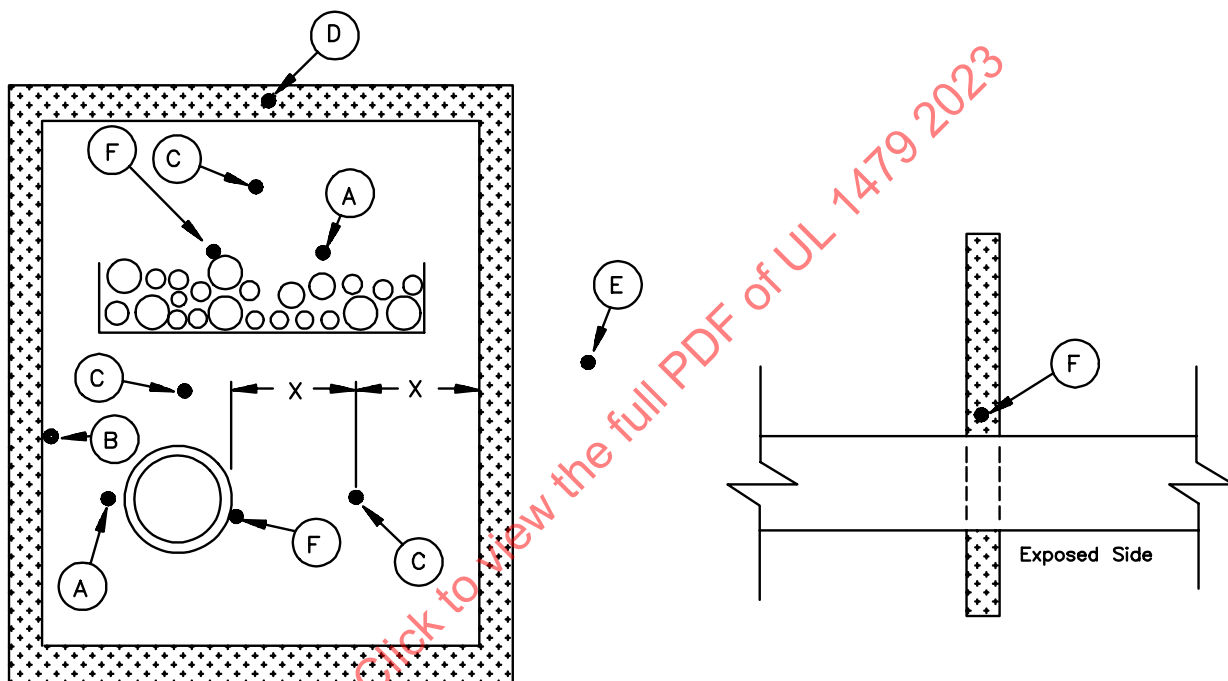
Figure 5.2 Temperature measurements locations a
