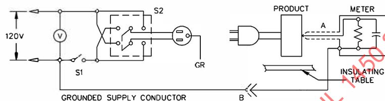
Figure 41.1 Leakage-current measurement circuits
