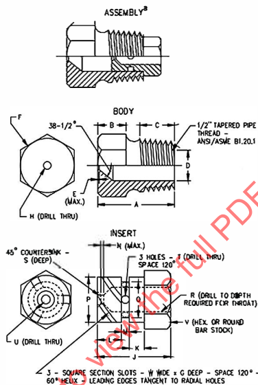
Figure 49.2 Spray-head assembly
