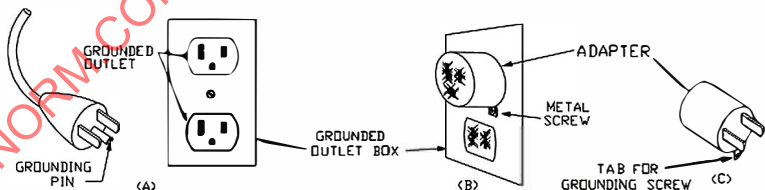
Figure 69.1 Grounding methods
