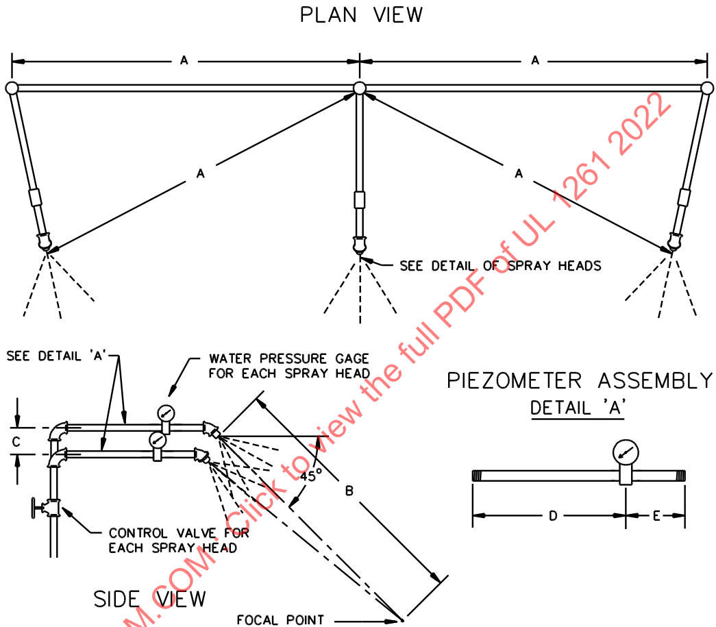
Figure 32.1 Spray head piping
