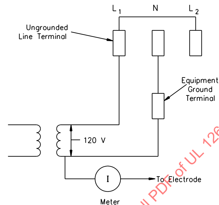
Figure 36.2 Test circuit connections
