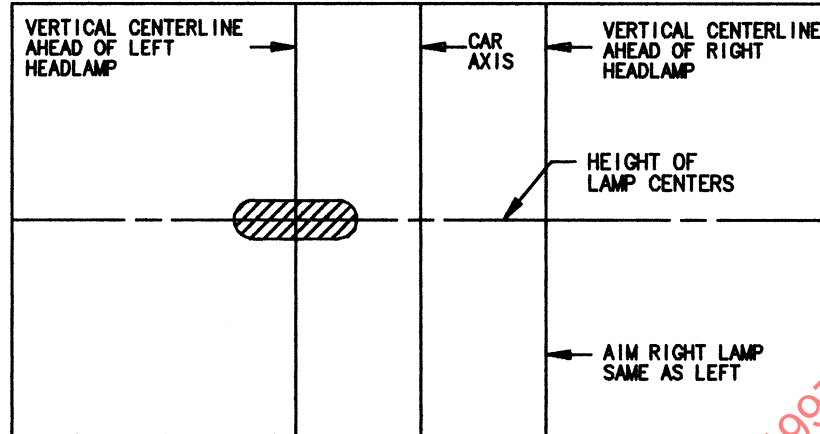
FIGURE 2—HIGH-INTENSITY ZONE (SHADED AREA OF A PROPERLY AIMED UPPER BEAM ON THE AIMING SCREEN 7.6 m (25 ft) IN FRONT OF VEHICLE
