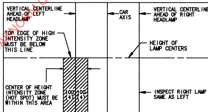
FIGURE 7—AIM INSPECTION LIMITS FOR SYMMETRICAL BEAM FOG LAMPS (UNIVERSAL MOUNTING APPLICATION)
