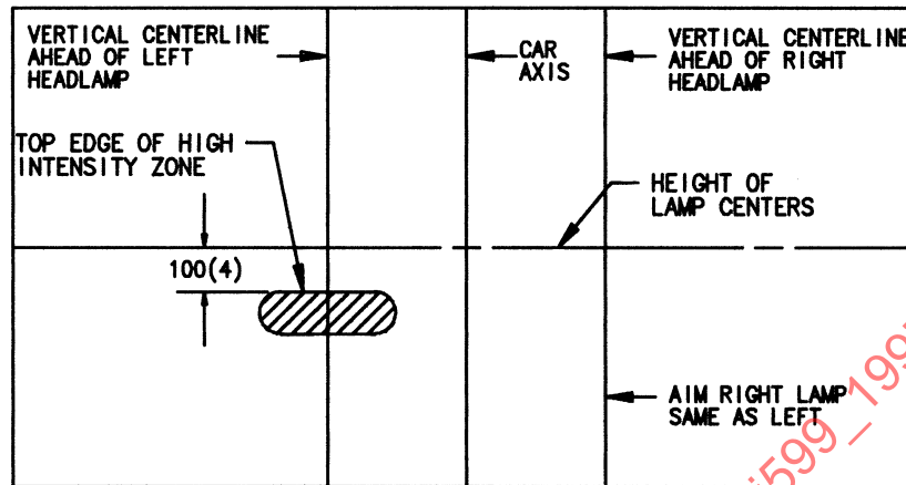
FIGURE 6—A PROPERLY AIMED SYMMETRICAL FOG LAMP BEAM (SHADED AREA INDICATES HIGH INTENSITY ZONE)
