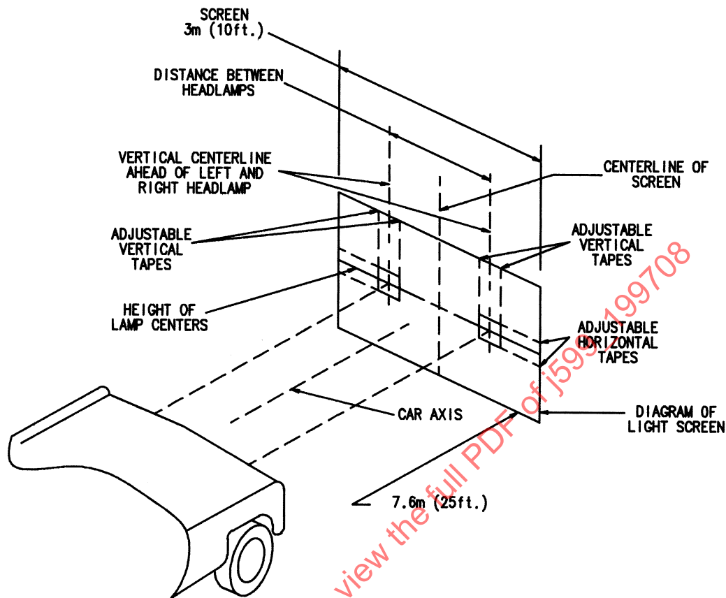
FIGURE 1—ALIGNMENT OF HEADLAMP AIMING SCREEN
