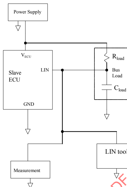
FIGURE 9—BROADCAST RESET SLAVE RESPONSE TEST SETUP
