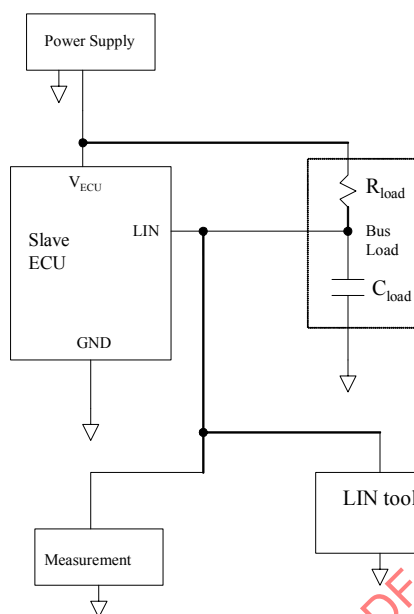
FIGURE 21—SLAVE NODE T_{r-d \max} AND T_{d-r \max} MEASUREMENT TEST SETUP
