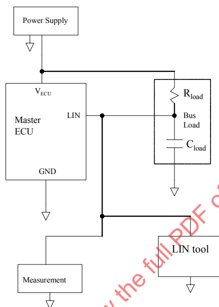
FIGURE 3—SLAVE TASK IN A MASTER NODE ERROR BEHAVIOR TEST SETUP
