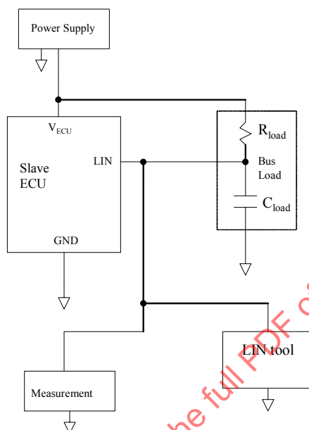
FIGURE 6—FIXED DNN TEST SETUP
