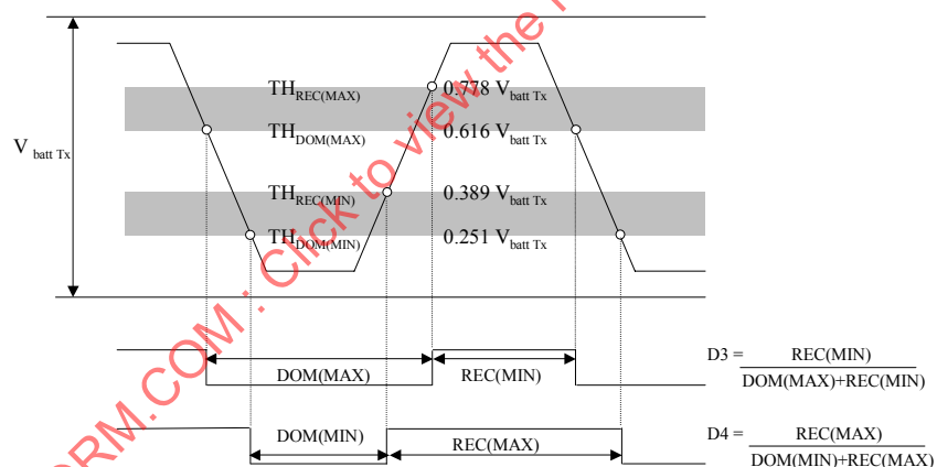
FIGURE 20— T_{r-d \max} AND T_{d-r \max} MEASUREMENT DESCRIPTION
