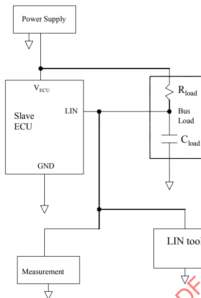
FIGURE 2—SLAVE NODE ERROR BEHAVIOR TEST SETUP
