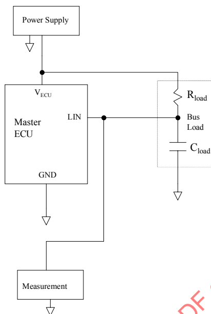
FIGURE 10—MASTER NODE BIT TIME MEASUREMENT TEST SETUP
