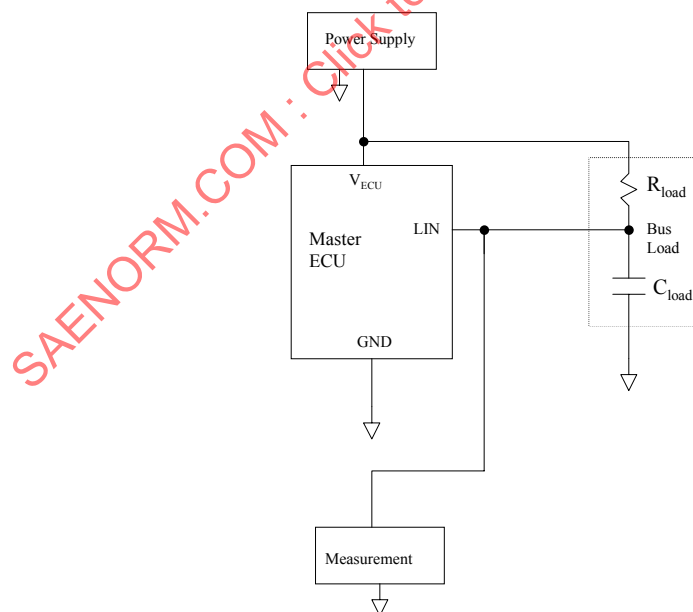
FIGURE 13—MASTER NODE V_{oh} AND V_{ol} LEVELS MEASUREMENT TEST SETUP
