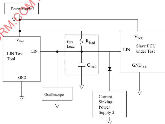
FIGURE 16—SLAVE NODE V_{ih} LEVEL MEASUREMENT TEST SETUP
