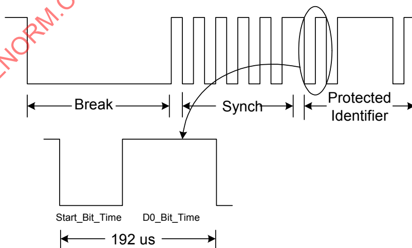
FIGURE 23—DOMINANT TO RECESSIVE EDGE SHIFTING DESCRIPTION
