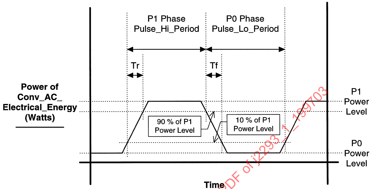
FIGURE 11—AC-TO-AC CONVERSION PULSE MODE TIMING
