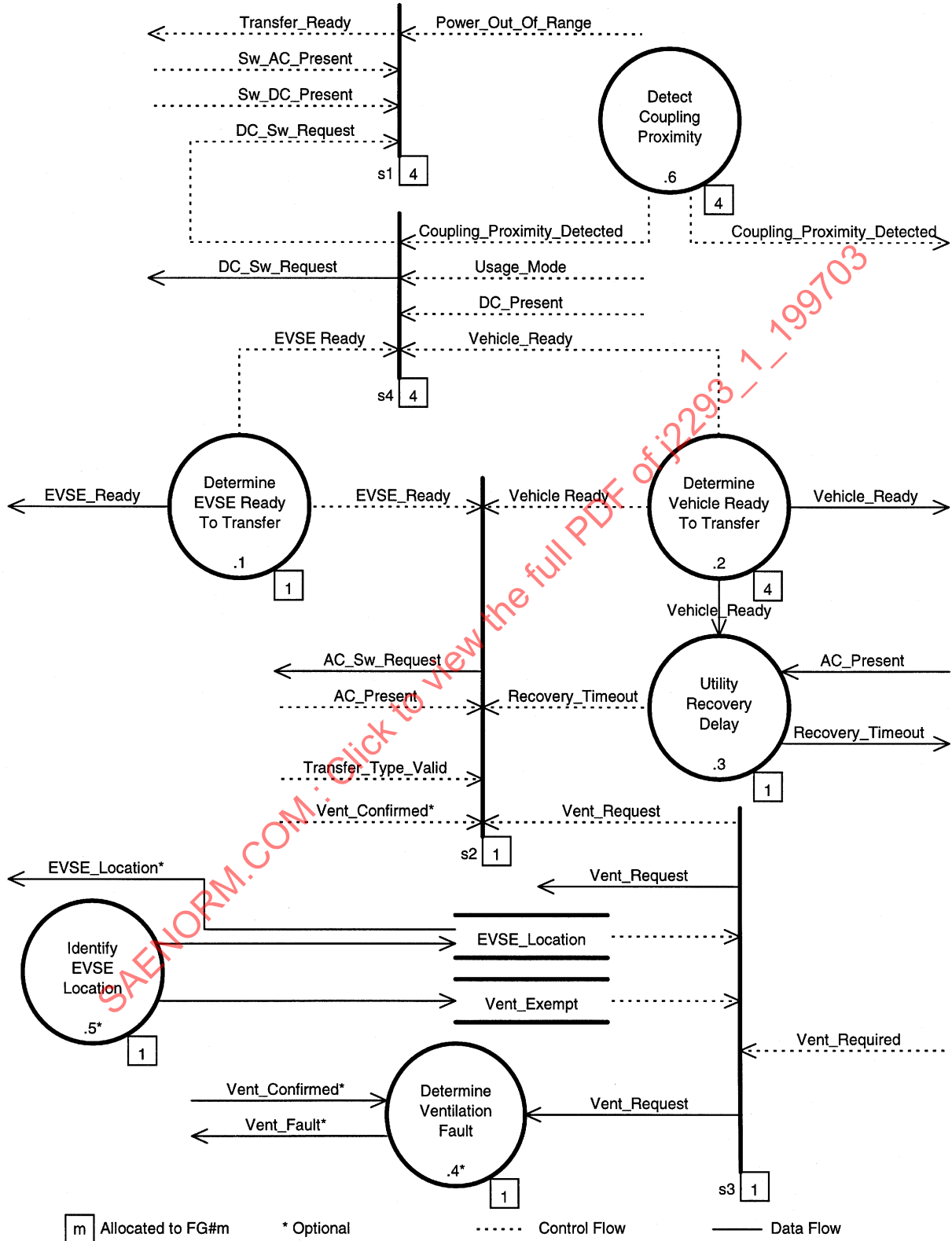
FIGURE 13—2.0: DETERMINE READY TO TRANSFER ELECTRICAL ENERGY DFD
