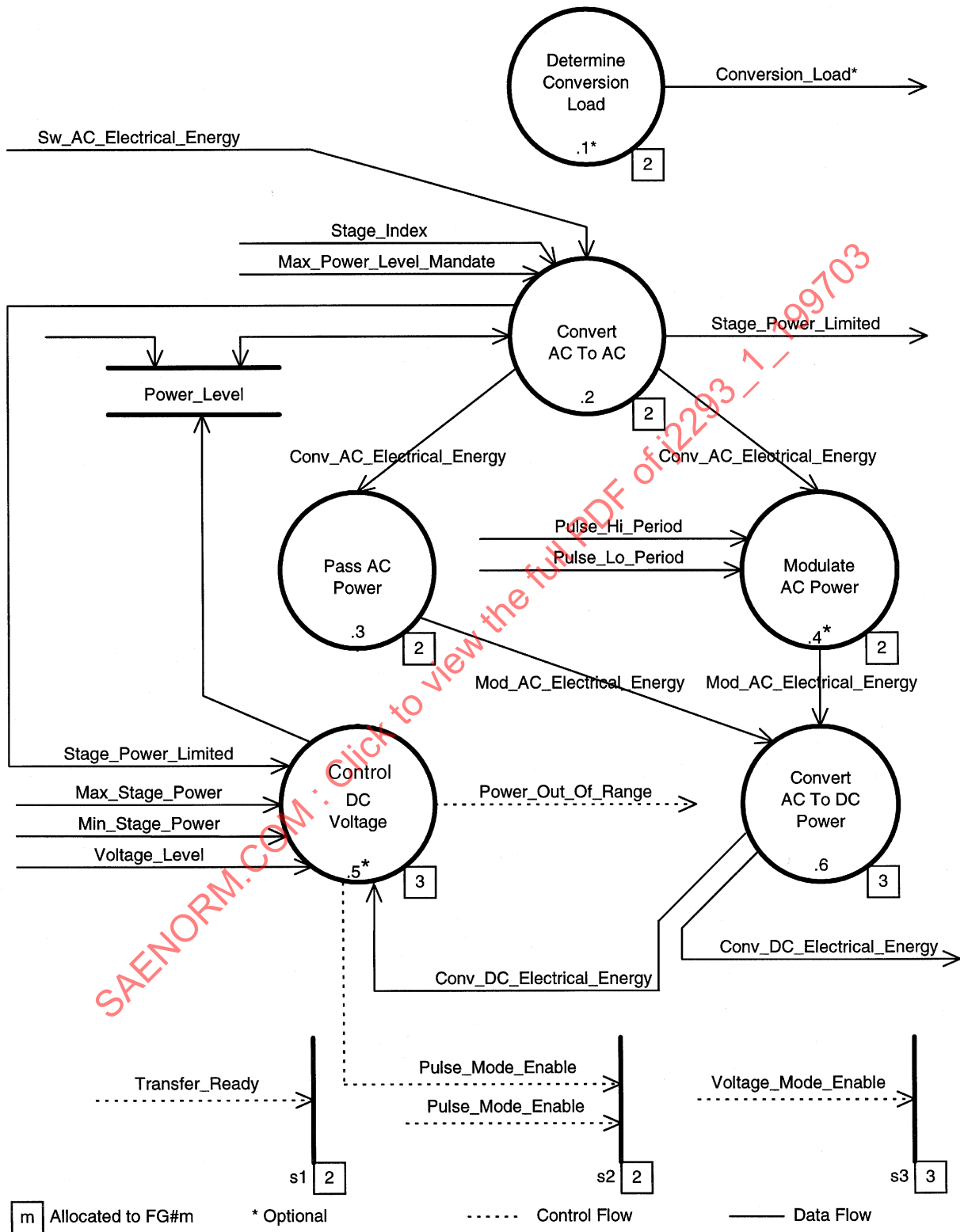
FIGURE 8—1.3: CONVERT AC TO DC DFD
