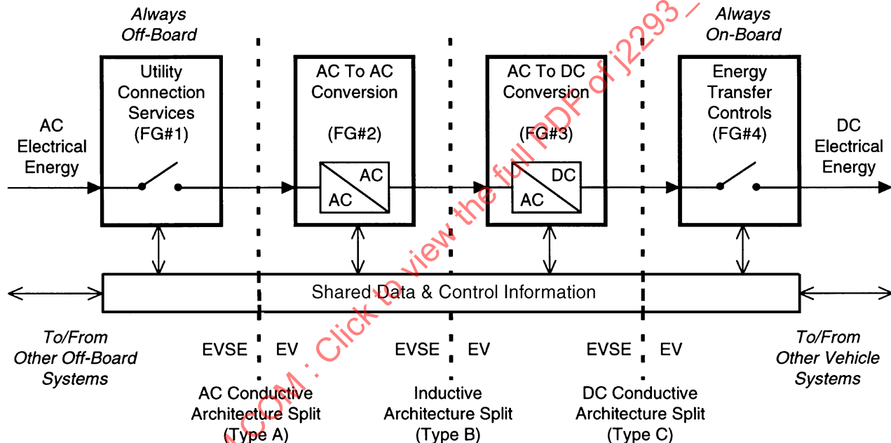
FIGURE 2—EV ETS FUNCTIONAL GROUP SERIES ENERGY CONVERSION
