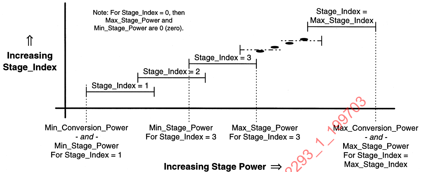
FIGURE 16—RELATIVE CONVERSION STAGE POWER RANGE
