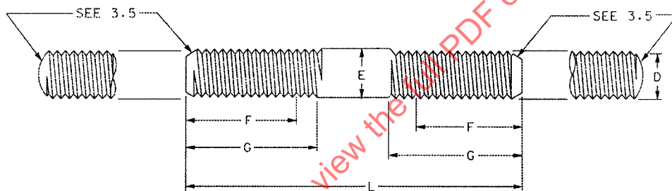
FIGURE 3—DOUBLE END STUD BOLTS—CLAMPING TYPE (REFER TO TABLE 1 FOR DIMENSIONS)
