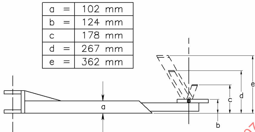
FIGURE 7A - FLIP-UP ADAPTER
