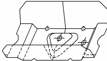
FIGURE 3 - TYPICAL LIFT POINT WITH TRIANGULAR BOSS/DEPRESSION
