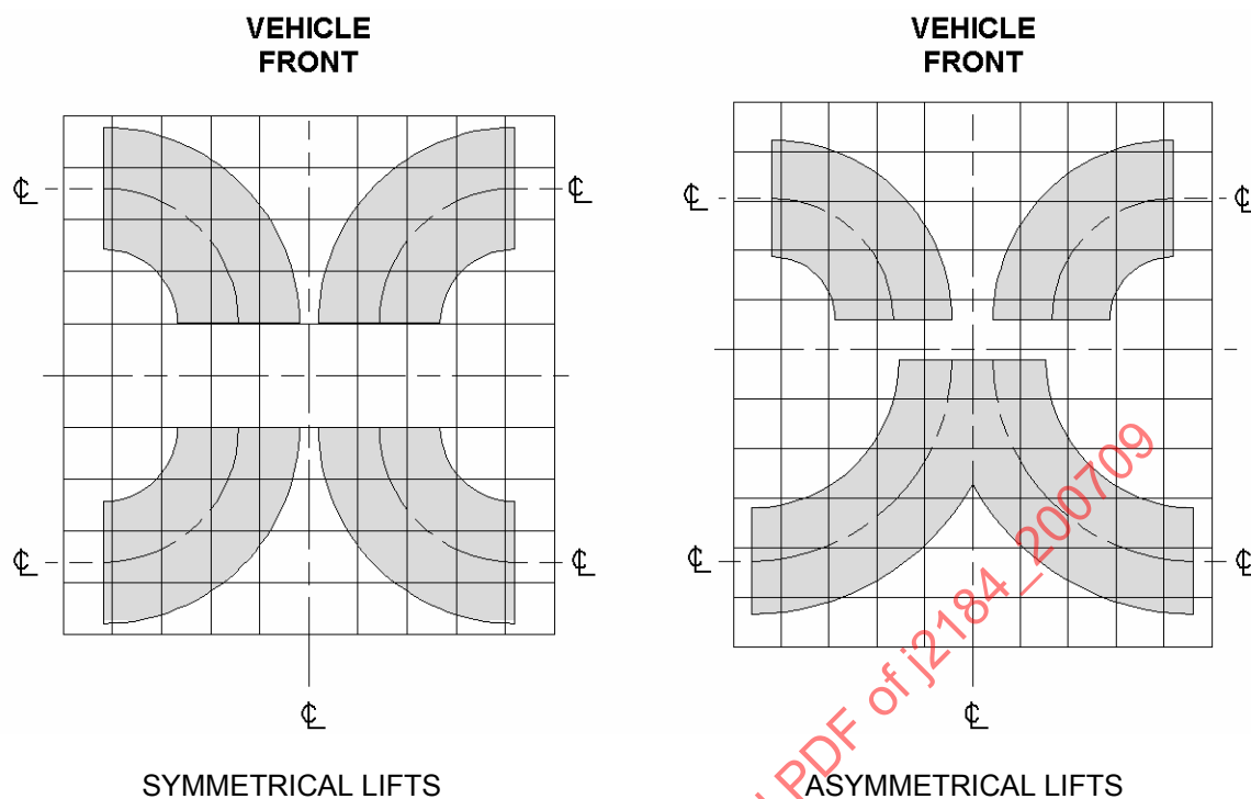
FIGURE 5 - ADAPTER ENVELOPE, SWING-ARM LIFTS Grid Line Spacing is 305 mm (12 in)
