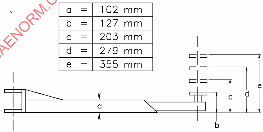
FIGURE 7C - STACKING ADAPTER
