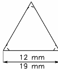
FIGURE 4 - LIFT POINT SYMBOL SIZE
