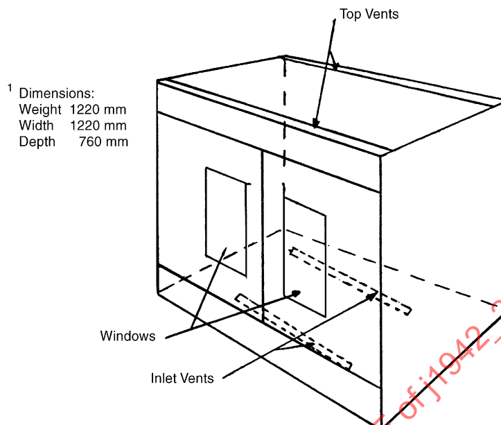
FIGURE 1—FIRE TEST CABINET
