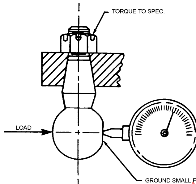
FIGURE 2—TEST FIXTURE
