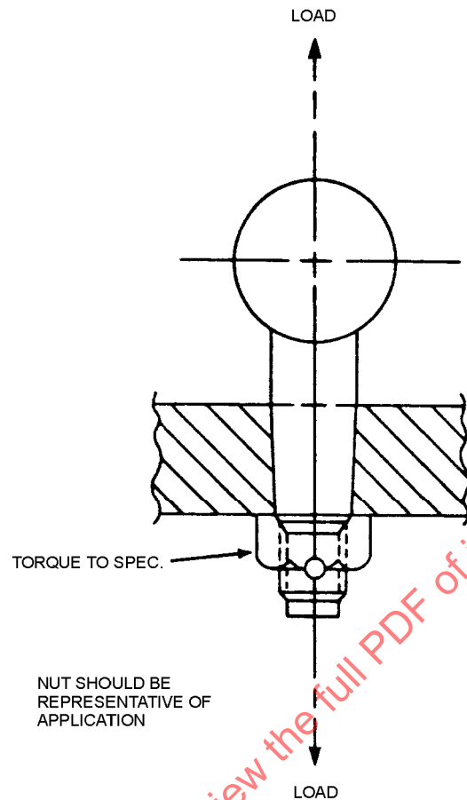
FIGURE 3—TENSILE TEST
