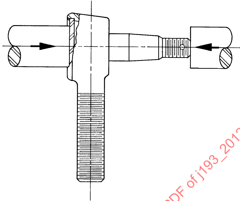
FIGURE 4A—BALL STUD TO SOCKET AXIAL END MOVEMENT—TYPICAL FIXTURE
