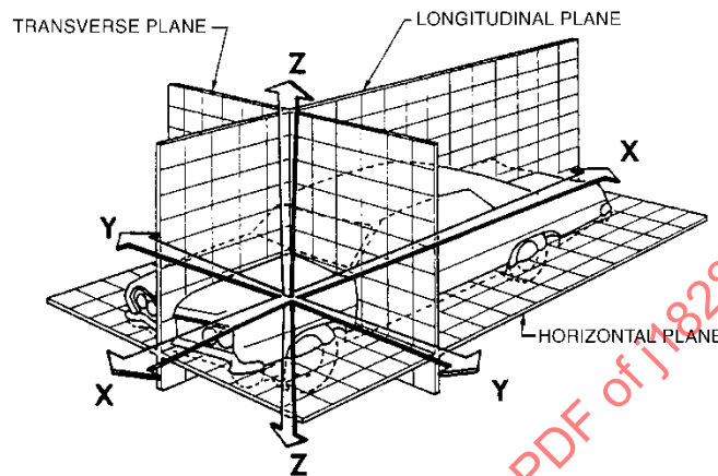
FIGURE 1 - DATUM PLANES
