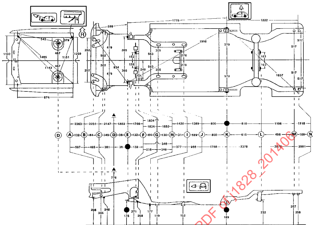
FIGURE 7 - SYMBOLS DEFINING DIRECTION OF VIEW
