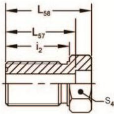
FIGURE 47 – BRAZE-ON BULKHEAD MALE TUBE (52M0173 & 52M01M73)
