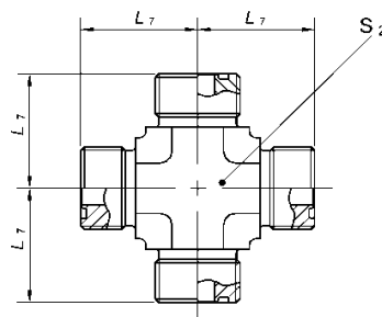
FIGURE 32 - UNION CROSS (52M0501)
