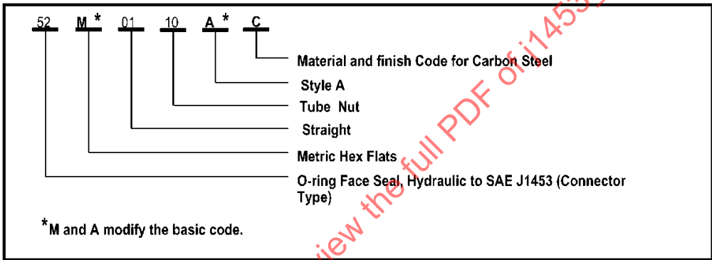
FIGURE 9 - CONNECTOR STYLE AND MATERIAL DESIGNATION
