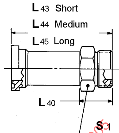
FIGURE 44B (SHORT – 52M3061 OR 52M3062) (MEDIUM – 52M3161 OR 52M3162) (LONG – 52M3261 OR 52M3262)
