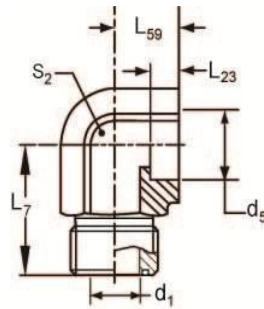
FIGURE 48 – BRAZE-ON 90°MALE TUBE (52M0373 & 52M03M73)
