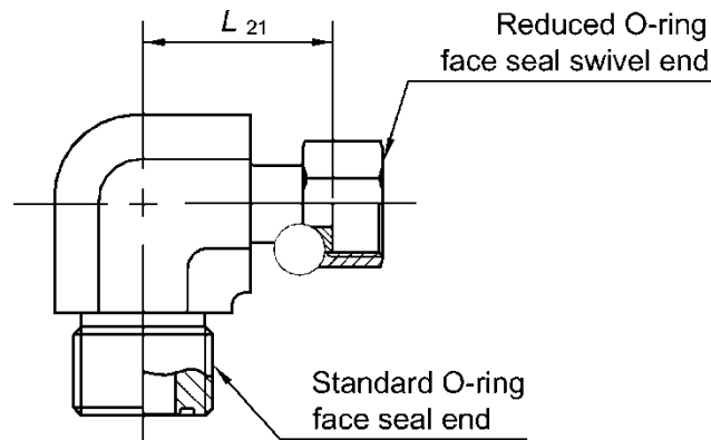
FIGURE A6 - SWIVEL ELBOW CONNECTOR WITH REDUCED SWIVEL END
