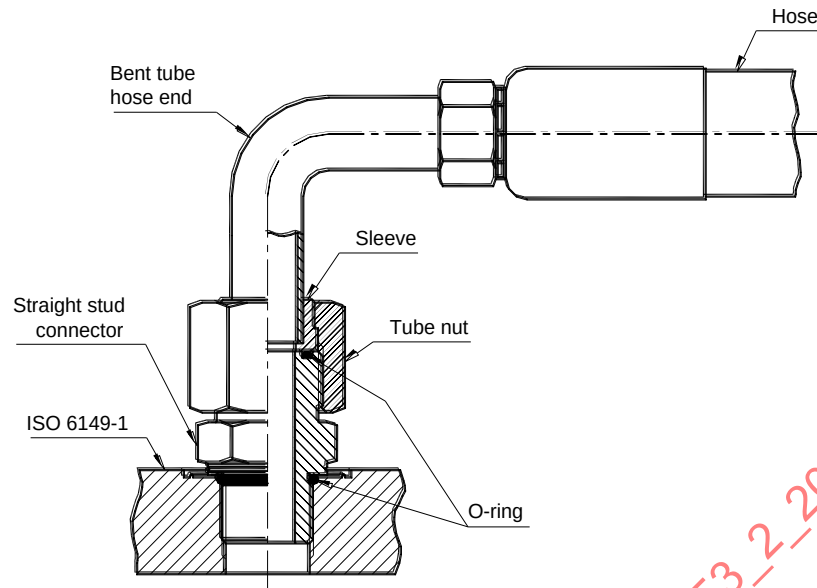
FIGURE 3 - TYPICAL CONNECTION – NON-ADJUSTABLE CONNECTOR TO HYDRAULIC HOSE
