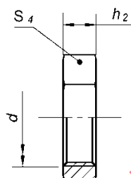
FIGURE 29 - BULKHEAD LOCKNUT (52M0118)
