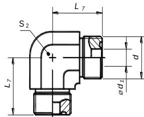
FIGURE 31 - 90° UNION ELBOW (52M0201)
