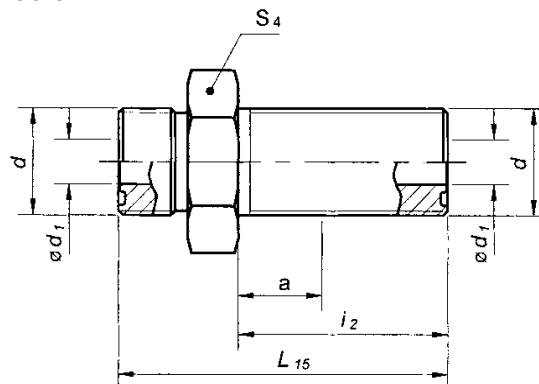
FIGURE 24 - BULKHEAD STRAIGHT (52M0601)
