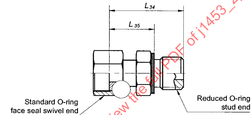
FIGURE A7B - STRAIGHT STUD SWIVEL WITH REDUCED STUD END
