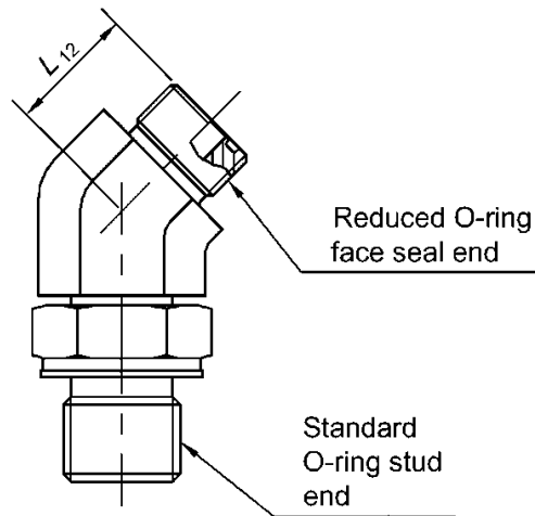
FIGURE A2A - 45 DEGREE ADJUSTABLE JUMP STUD ELBOW WITH REDUCED ORFS END
