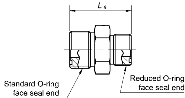
FIGURE A5 - STRAIGHT UNION CONNECTOR WITH ONE END REDUCED
