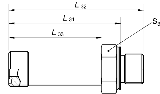
FIGURE 23 - STUD STRAIGHT LONG (52M1787)
