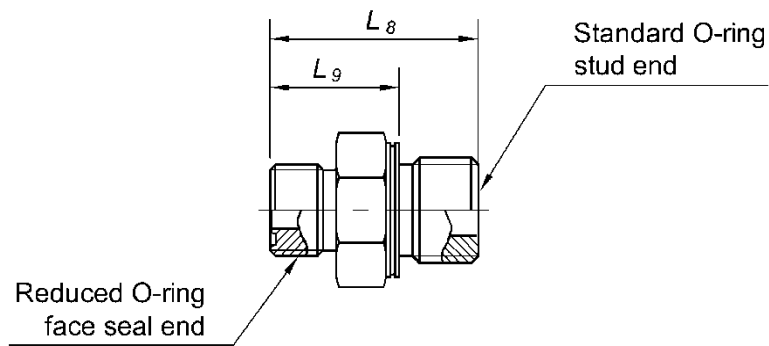
FIGURE A3A - STRAIGHT-STUD CONNECTOR WITH REDUCED ORFS END
