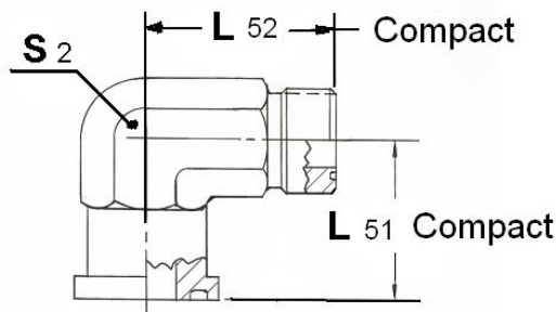
FIGURE 46A (COMPACT – 52M3461 OR 52M3462)
