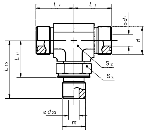
FIGURE 18 - ADJUSTABLE STUD BRANCH TEE (52M0489)
