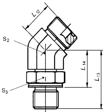
FIGURE 17 - 45 DEGREE ADJUSTABLE STUD ELBOW (52M0387)
