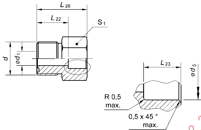
FIGURE 39 - BRAZE-ON STRAIGHT (52M0172), (52M01M72, METRIC TUBING)
