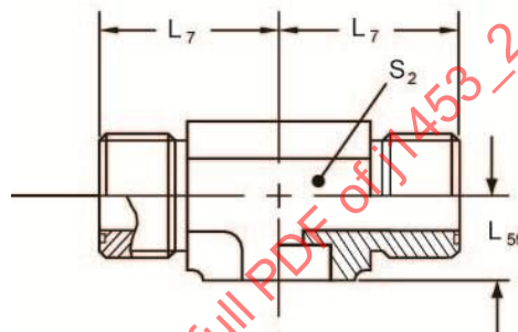
FIGURE 48 – BRAZE-ON 90°MALE TUBE (52M0373 & 52M03M73)
