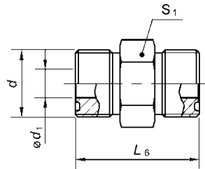
FIGURE 30 - UNION STRAIGHT (52M0101)
