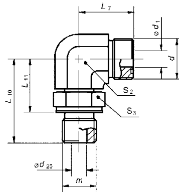
FIGURE 15 - 90 DEGREE ADJUSTABLE STUD ELBOW (52M0287)
