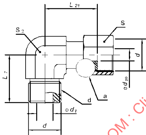
FIGURE 33 - SWIVEL 90 DEGREE ELBOW (52M0221)
