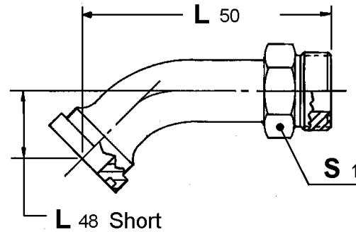
L 49 Medium FIGURE 45B (SHORT – 52M2261 OR 52M2262) (MEDIUM – 52M2361 OR 52M2362)
