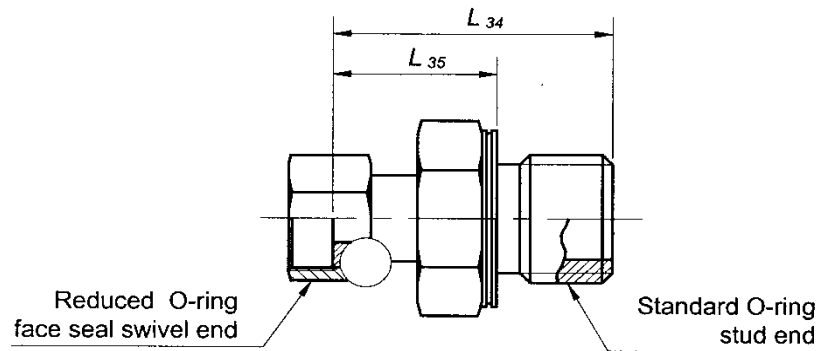
FIGURE A7A - STRAIGHT STUD SWIVEL WITH REDUCED SWIVEL END
