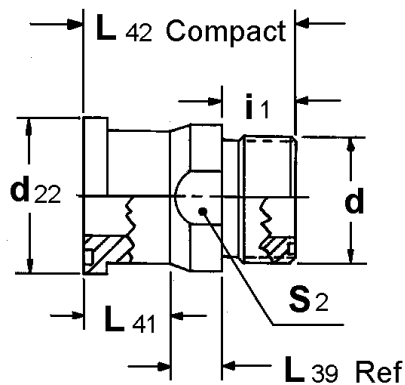
FIGURE 44A (COMPACT – 52M2961 OR 52M2962)
