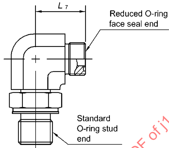
FIGURE A1A - 90 DEGREE ADJUSTABLE JUMP STUD ELBOW WITH REDUCED ORFS END
