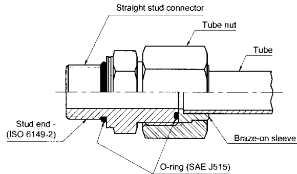
FIGURE 1 - TYPICAL REPRESENTATION OF O-RING FACE SEAL (ORFS) CONNECTION (SEE SAE J1453-3 FOR SAE J1926-2 INCH STUD END PARTS.)
