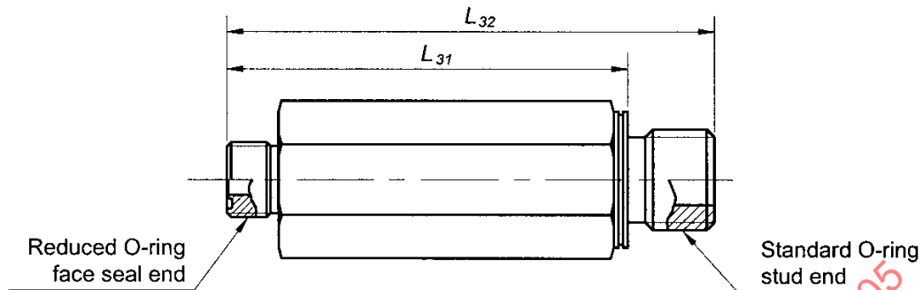
FIGURE A4A - LONG STRAIGHT STUD CONNECTOR WITH REDUCED ORFS END
