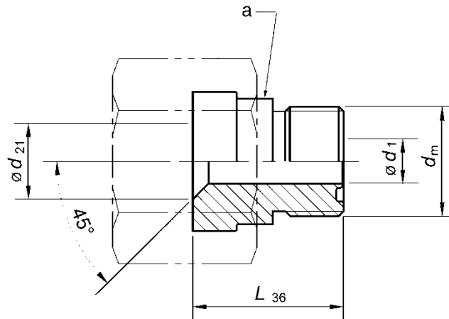
FIGURE 43 - REDUCER WITHOUT NUT (STYLE B) (520123B)
