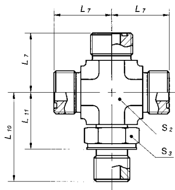
FIGURE 20 - ADJUSTABLE STUD CROSS (52M0587)
