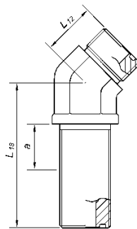
FIGURE 27 - 45 DEGREE BULKHEAD ELBOW (52M0801)
