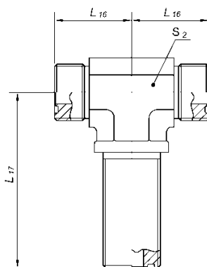
FIGURE 28 - BULKHEAD BRANCH TEE (52M0959)
