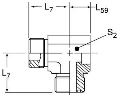
FIGURE 49 – BRAZE-ON MALE TUBE RUN TEE ADAPTER ( 52M0483 & 52M04M83)
