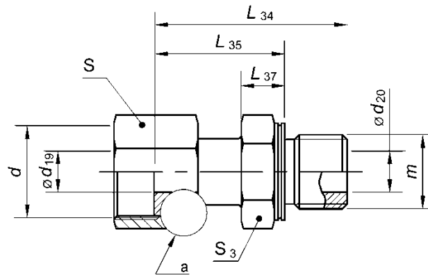
FIGURE 38 - STUD STRAIGHT SWIVEL (52M0196)
