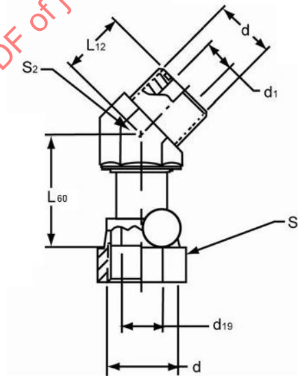
FIGURE 34 - SWIVEL 45 DEGREE ELBOW (52M0321)
