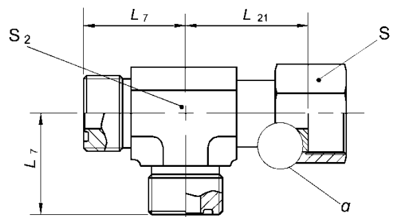
FIGURE 36 - SWIVEL RUN TEE (52M0432)
