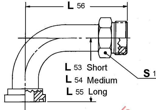
FIGURE 46B (SHORT – 52M1461 OR 52M1462) (MEDIUM – 52M2061 OR 52M2062) (LONG – 52M1561 OR 52M1562)
