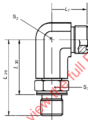
FIGURE 16 - 90 DEGREE ADJUSTABLE STUD ELBOW, LONG (52M1587)
