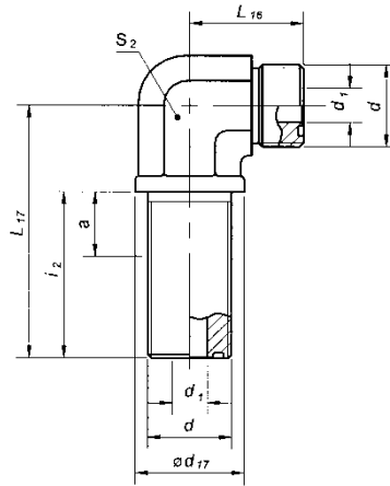
FIGURE 25 - 90 DEGREE BULKHEAD ELBOW (52M0701)
