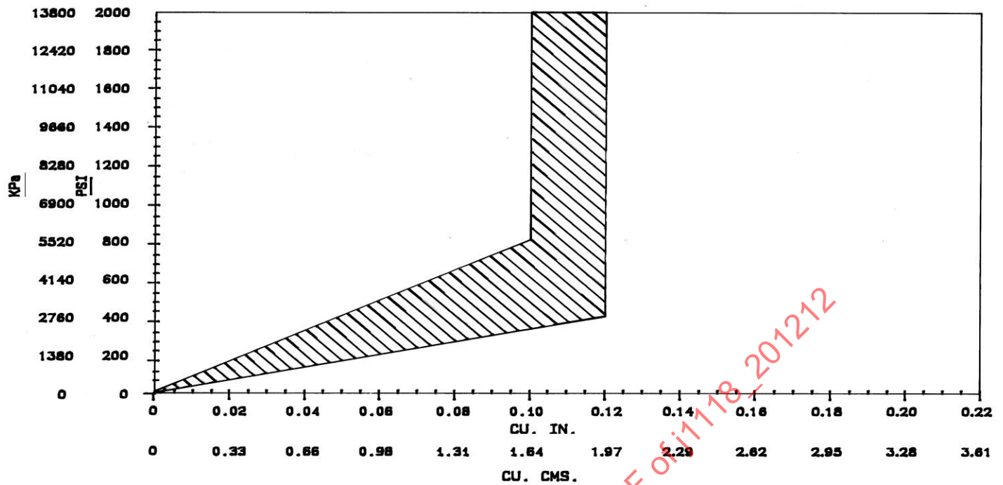
FIGURE 3—REAR BRAKES
