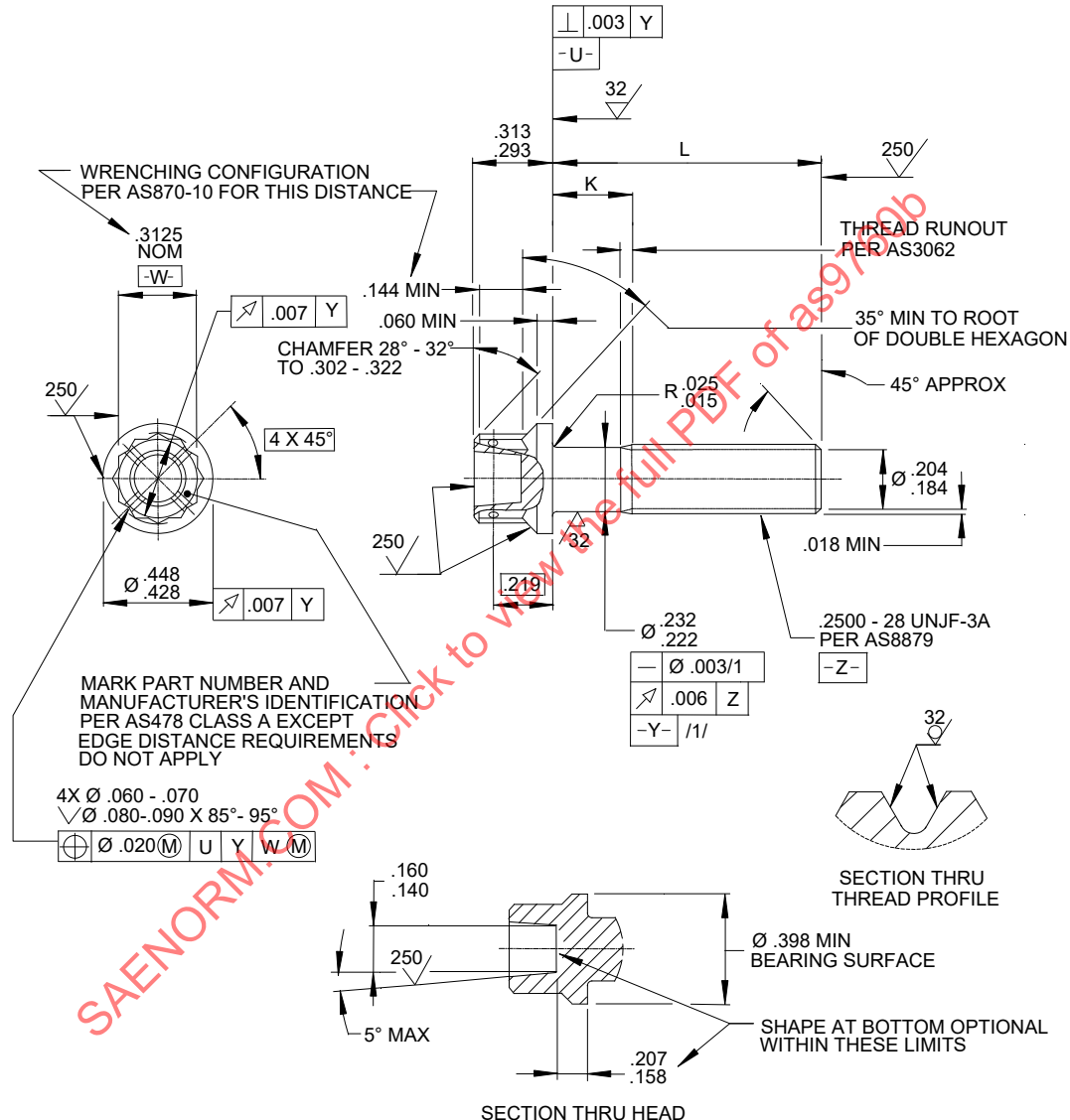
FIGURE 1 - BOLT
