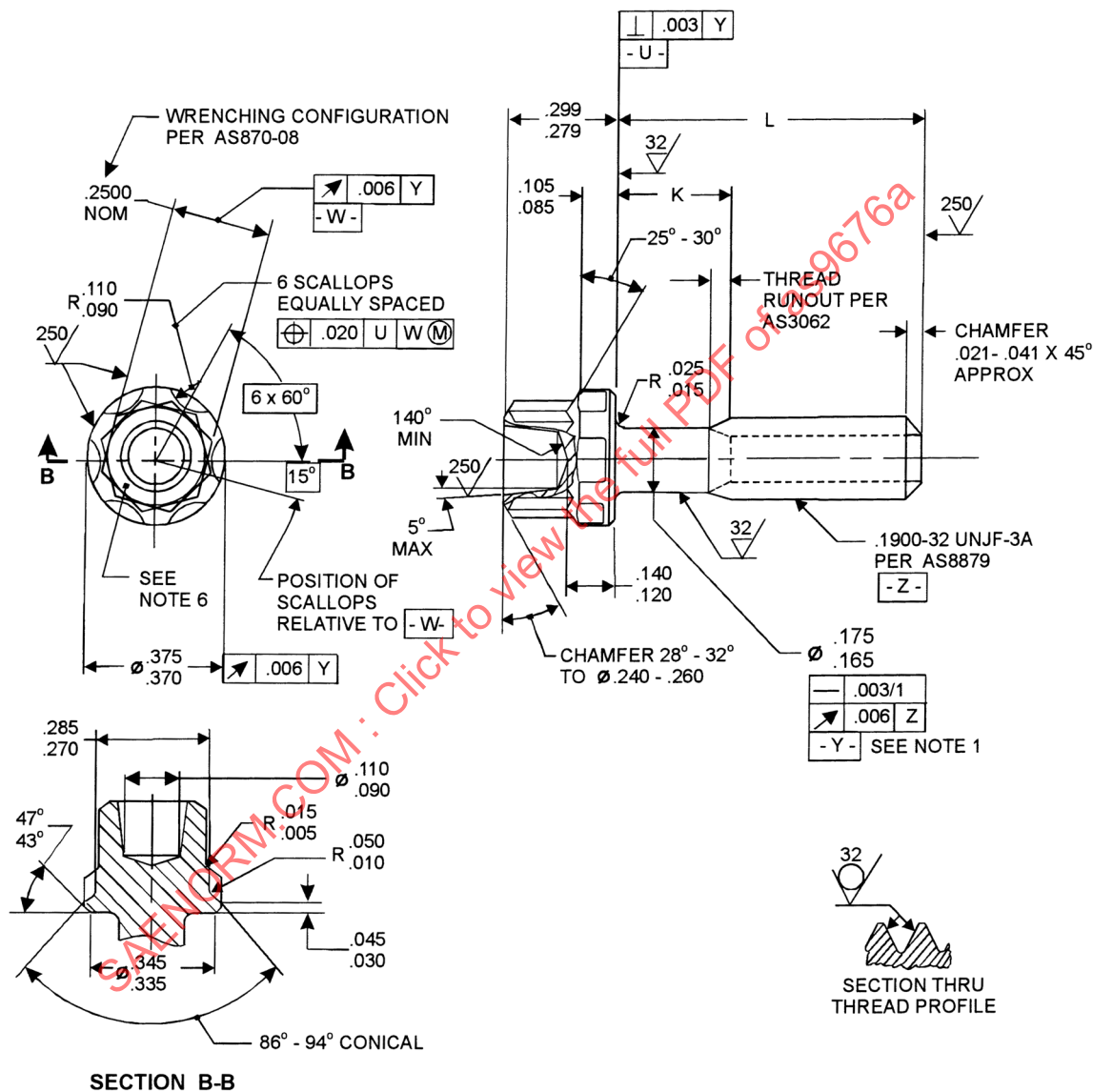
FIGURE 1 - BOLT
