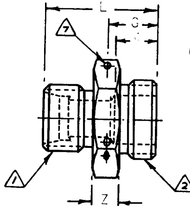
EXPANDER ADAPTER
