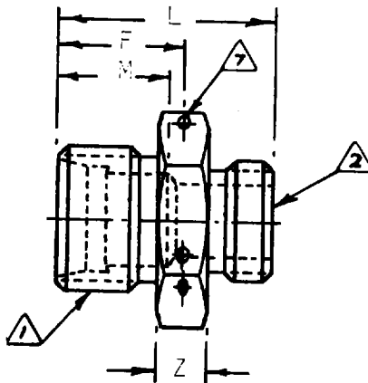
REDUCER ADAPTER
