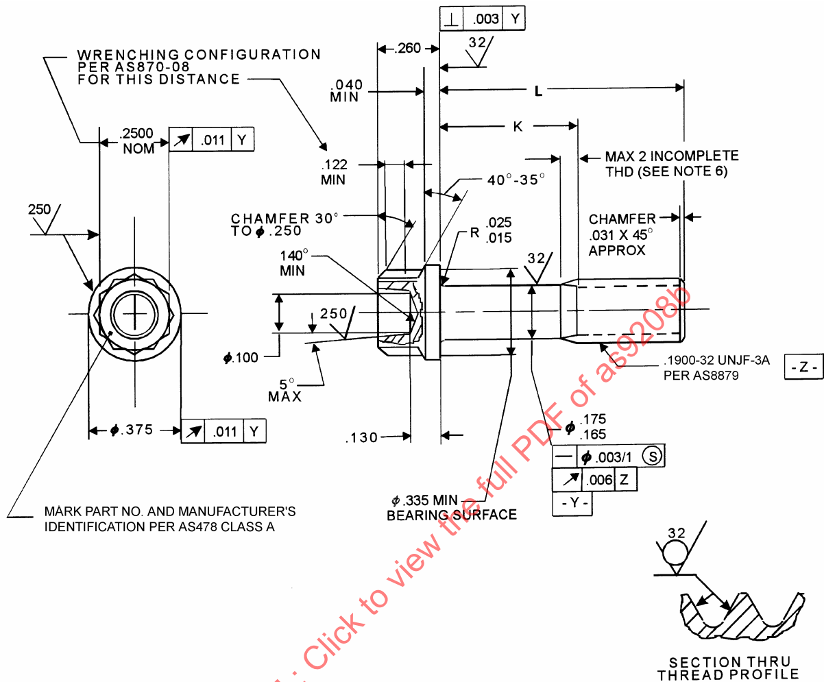
FIGURE 1 - BOLT
