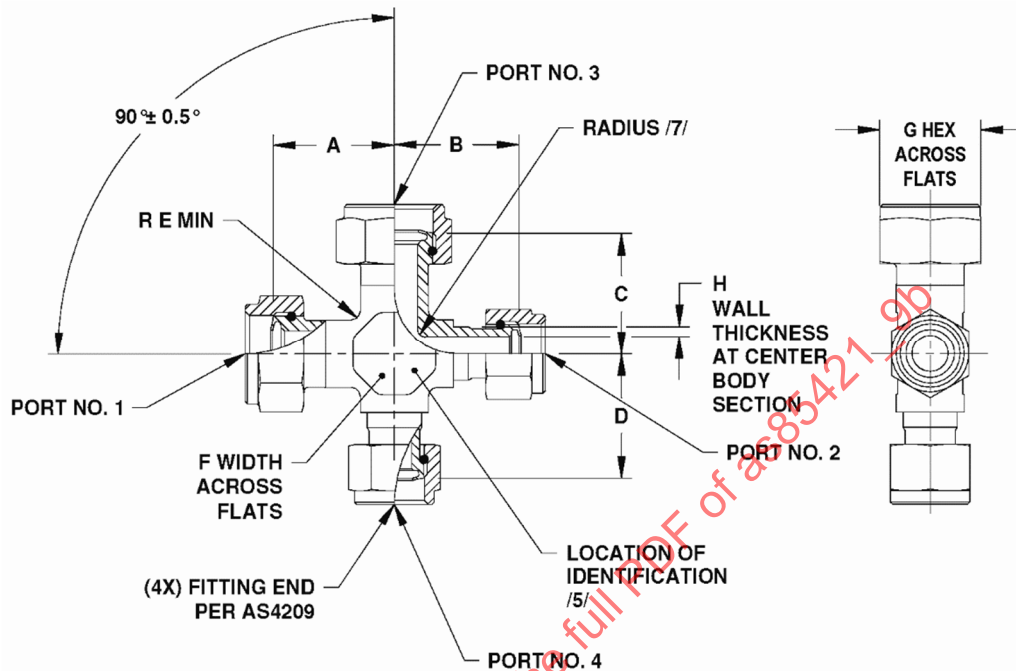
FIGURE 1 - FITTING ASSEMBLY, CROSS, REDUCER
