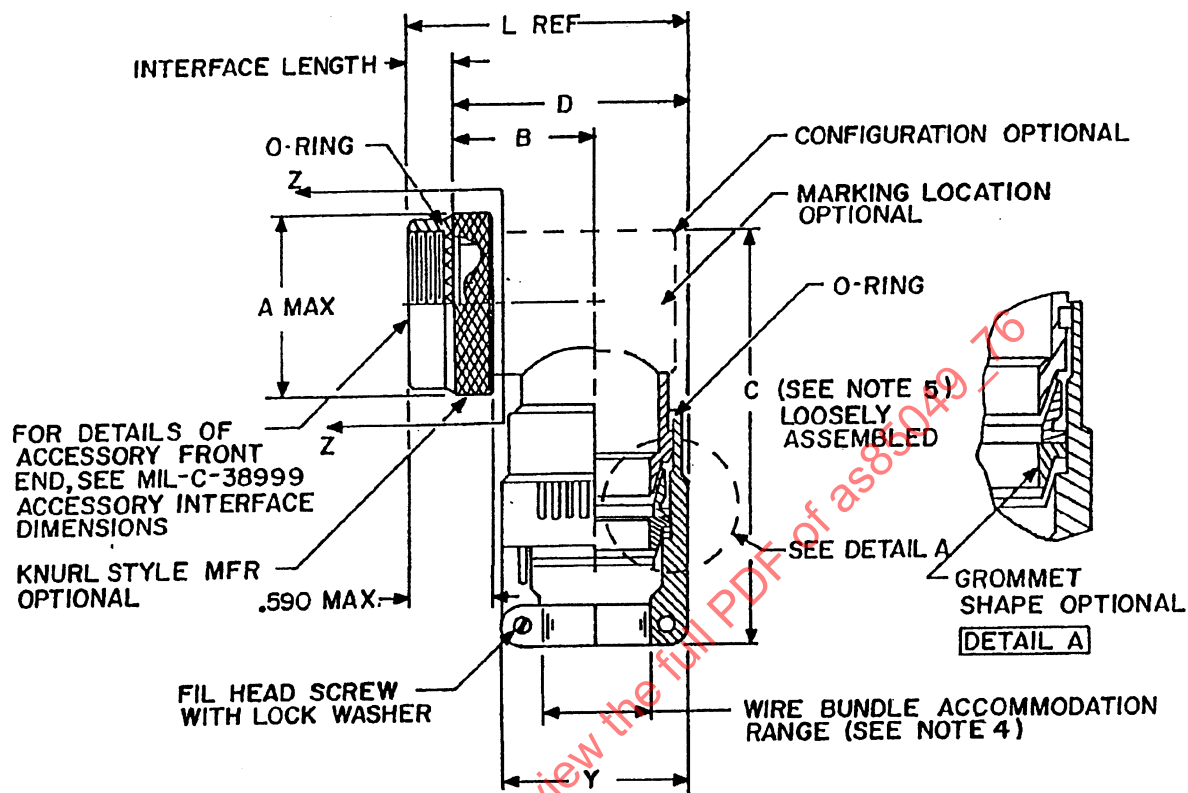
FIGURE 1. CONFIGURATIONN AND DIMENSIONS.
