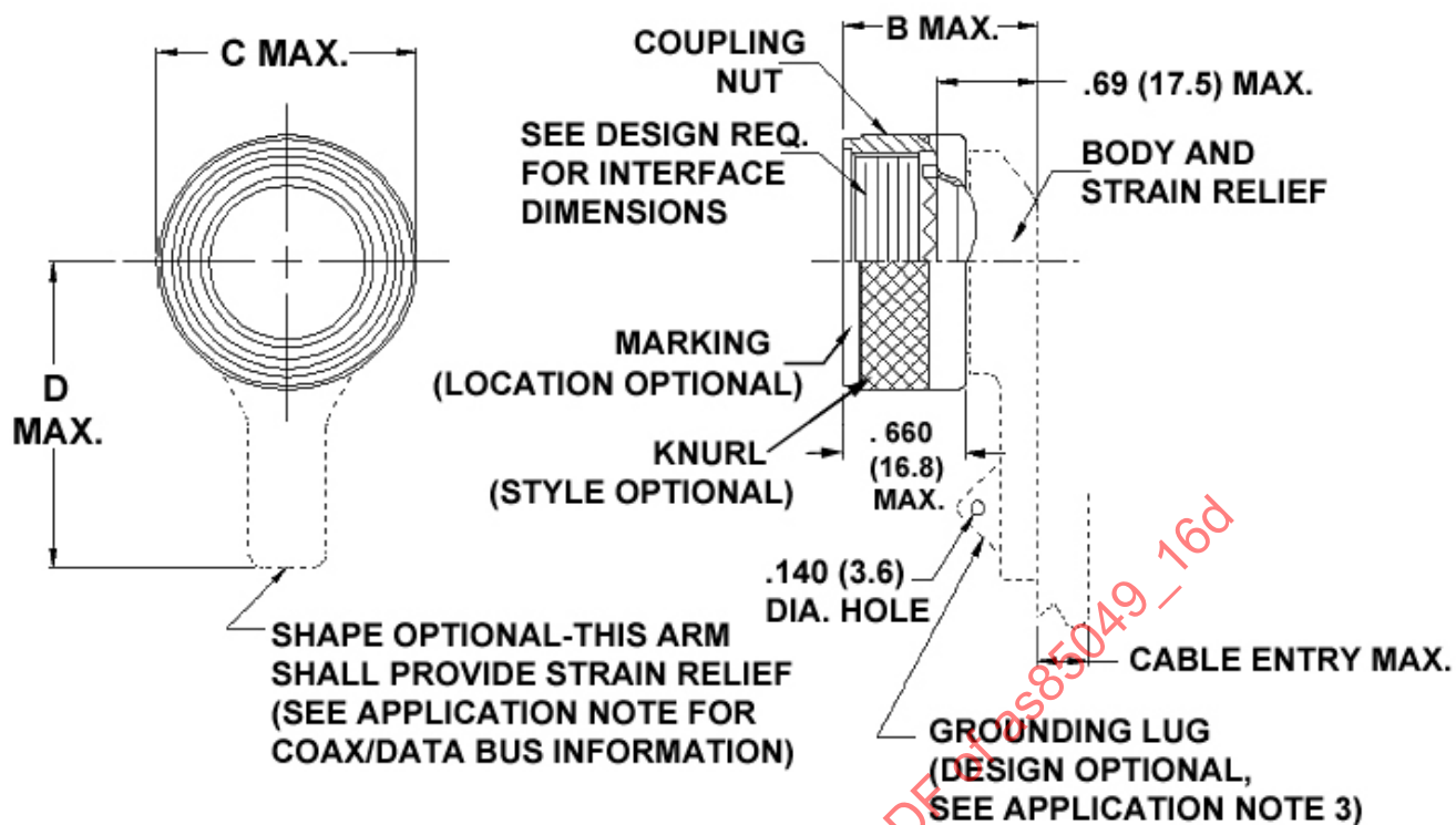
FIGURE 2 - ACCESSORY DIMENSIONS AND CONFIGURATION (SELF-LOCKING ONLY WITH GROUND LUG)
