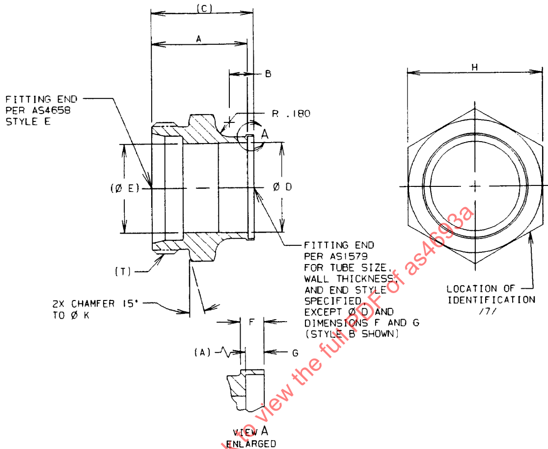
FIGURE 1 - UNION, TUBE END
