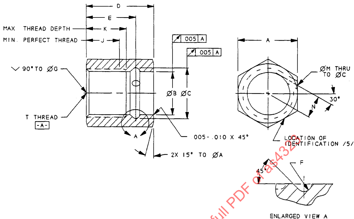
FIGURE 1 - SWIVEL NUT
