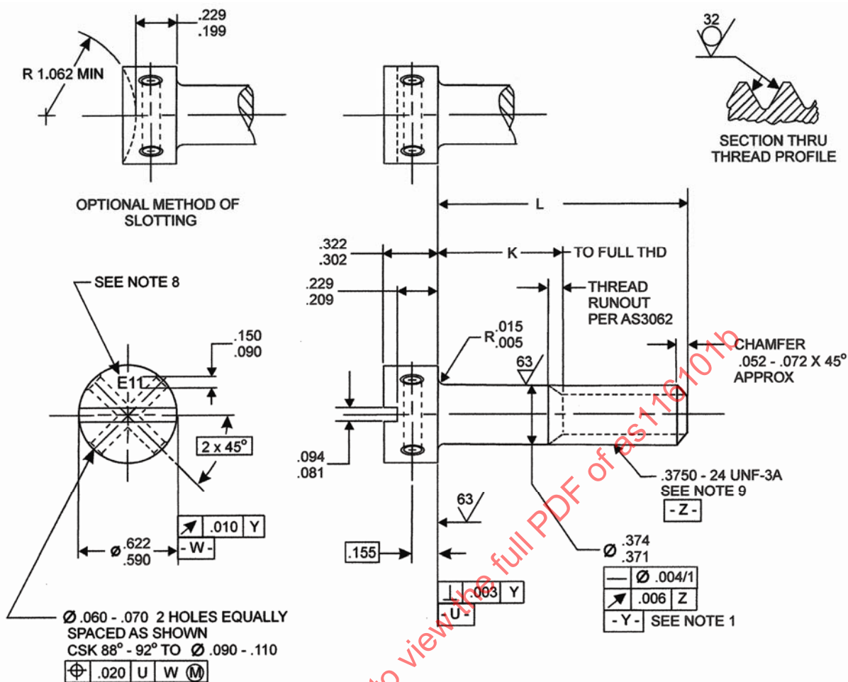
FIGURE 1 - SCREW
