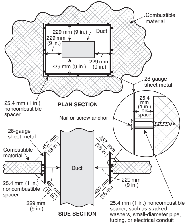
FIGURE A.4.2(f) Example of Clearance Reduction System: 229 mm (9 in.) Clearance to Combustible Material.
