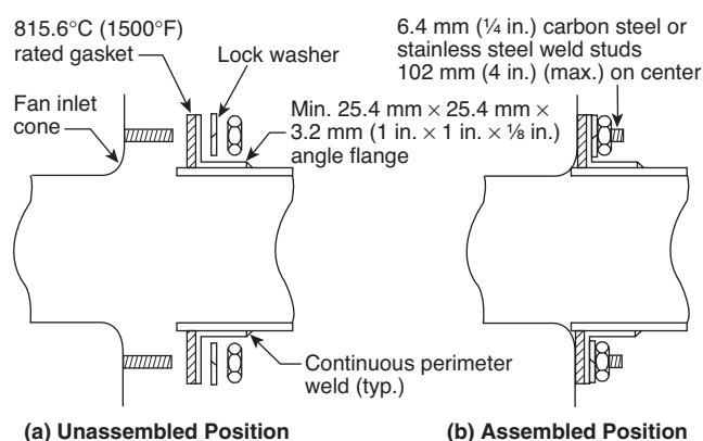
FIGURE 8.1.2.2(d) Typical Section of Duct-to-Fan Connection — Direct to Fan Inlet Cone Method.
