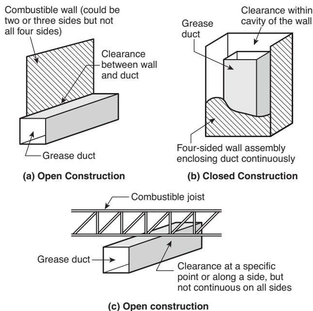
FIGURE A.3.3.13 Examples of Open and Closed Combustible Construction.
