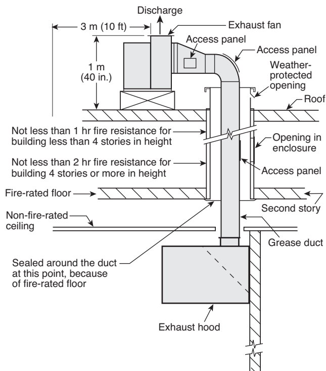
FIGURE A.4.2(c) Typical Section View for Building with Two Stories or More with Non-Fire-Rated Ceiling and Fire-Rated Floor. (Clearance notes in Figure A.4.2(a) apply also to this drawing.)
