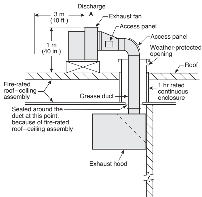
FIGURE A.4.2(b) Typical Section View for One-Story Building with Fire-Rated Roof-Ceiling Assembly. (Clearance notes in Figure A.4.2(a) apply also to this drawing.)
