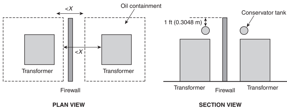
FIGURE 5.2.2.4 Outdoor Oil-Insulated Transformer Separation Criteria.
