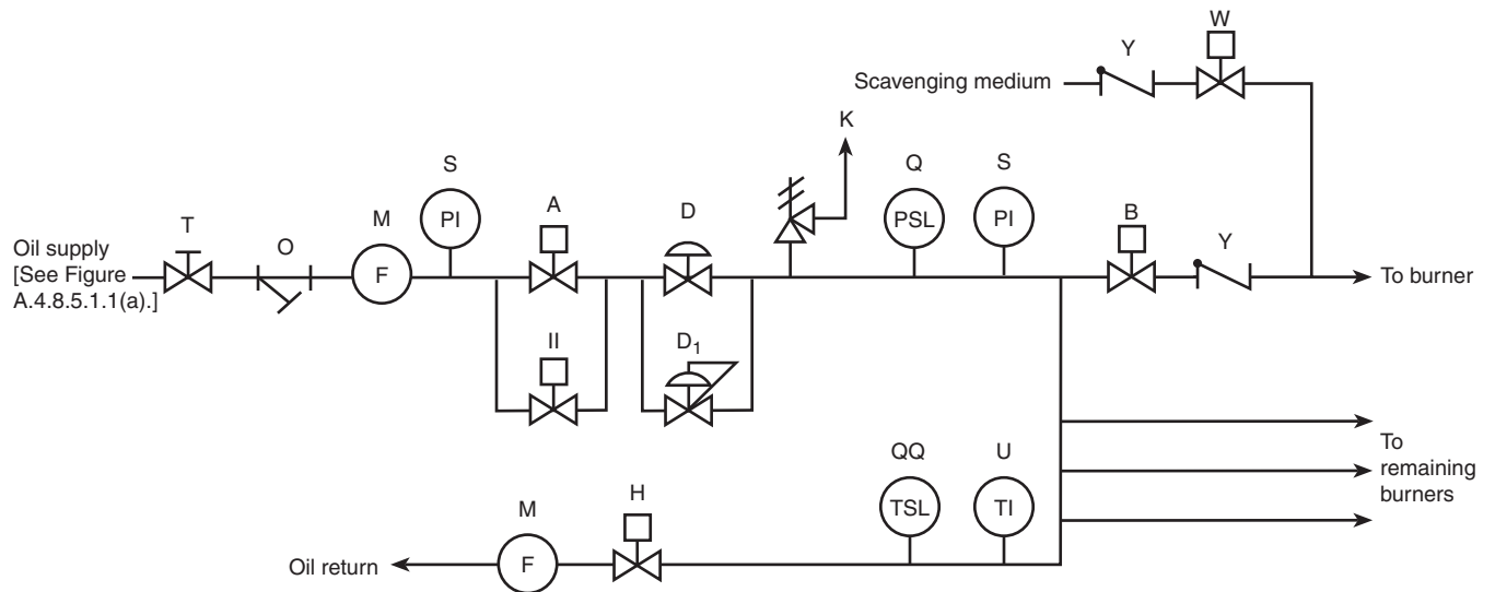
FIGURE A.4.8.5.1.1(e) Typical oil burner/lance system — mechanically atomized master fuel control valve for multiple burners (automatic).
