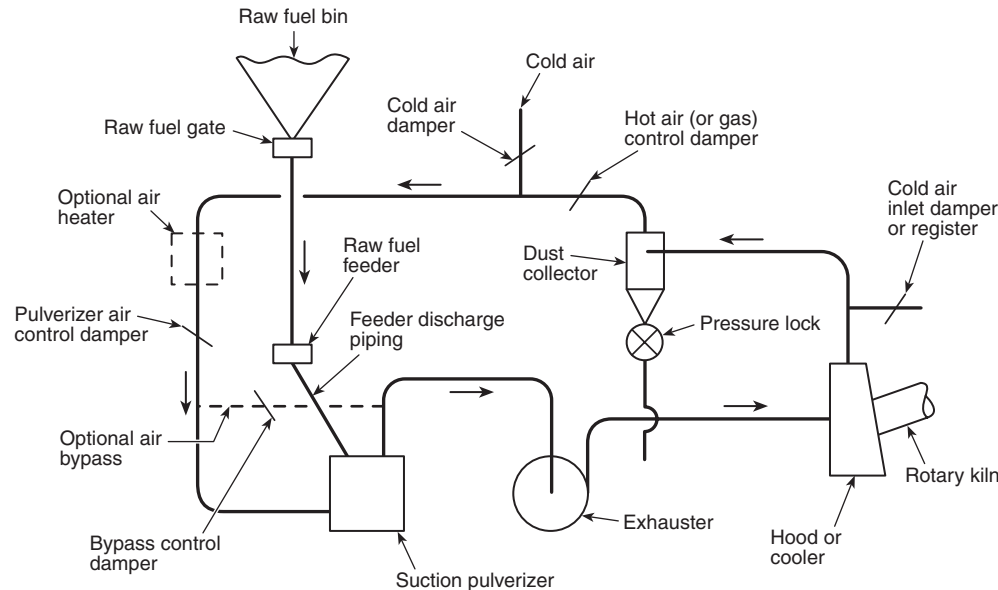
FIGURE 6.6.4.1(b) Direct-fired pulverized fuel systems for rotary kilns (with suction pulverizer).
