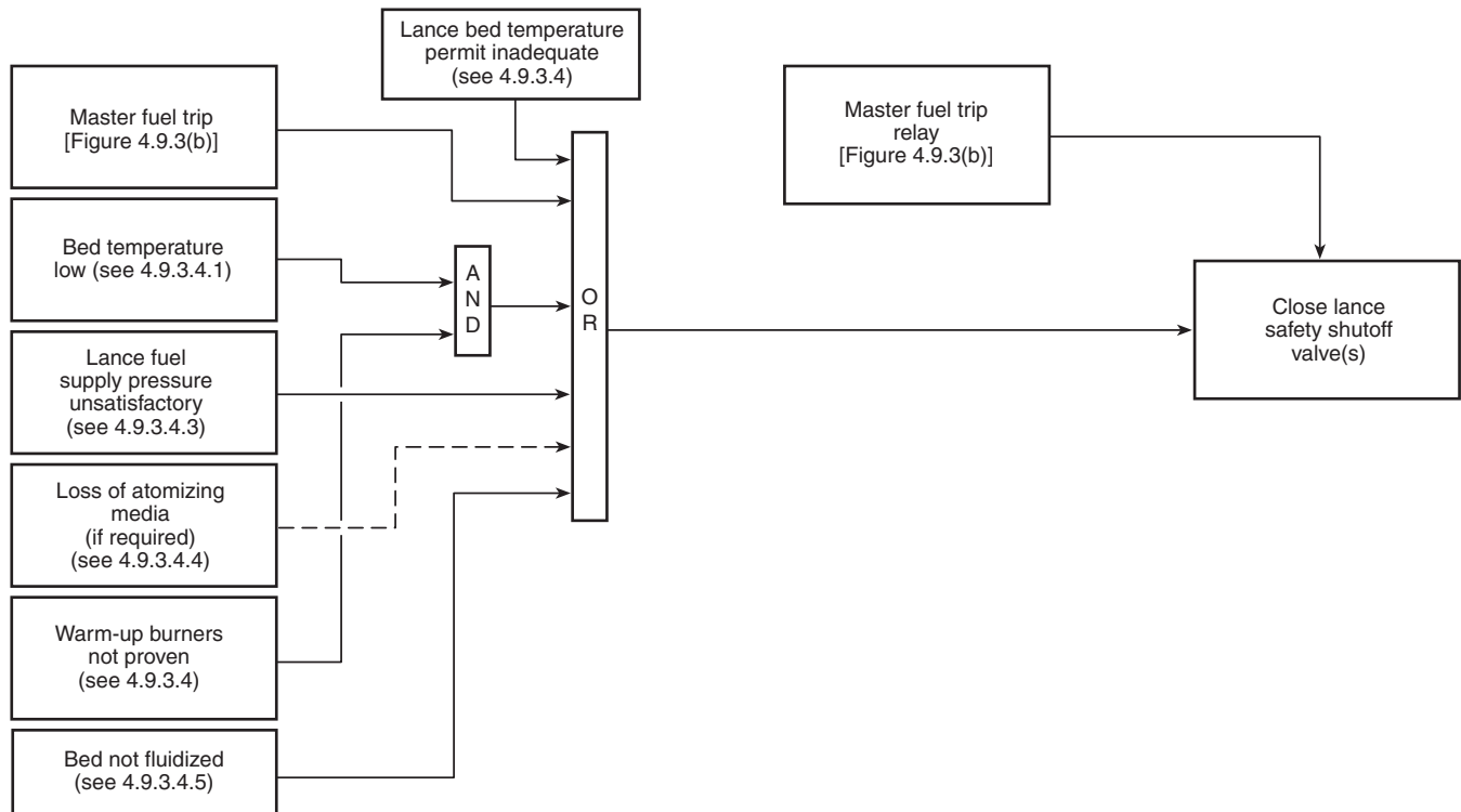
FIGURE 4.9.3(e) Lance safety subsystem.
