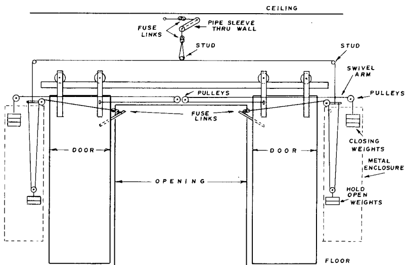
Figure A-39. Closing devices for center parting horizontally sliding doors (level track.)
