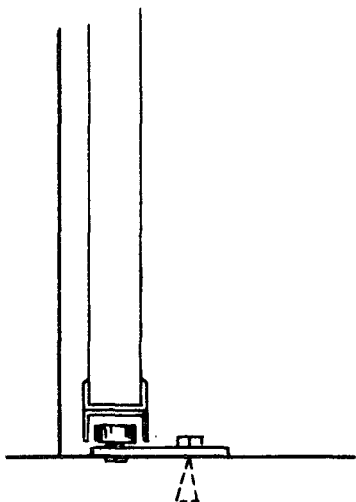
Figure A-15A Stay rolls.
