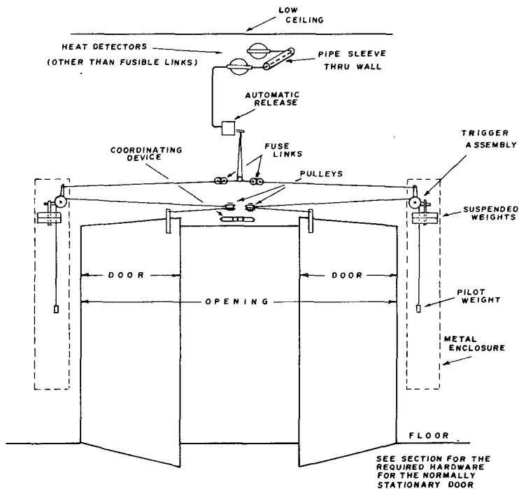
Figure A-32. Closing devices for doors swinging in pairs.
