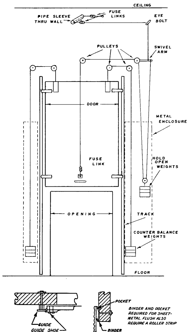
Figure A-45. Vertically sliding door.
