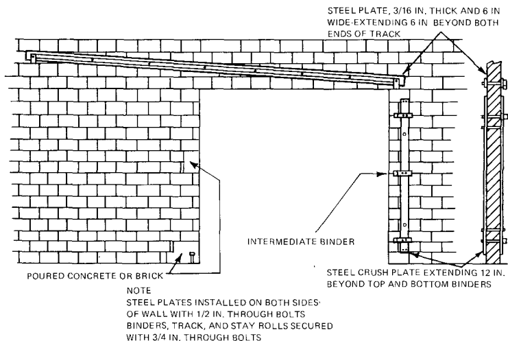
Figure A-19. Hollow concrete masonry wall prepared for a single sliding door. This illustrates typical reinforcement for anchorage of door-mounting hardware by use of steel plates to bridge the cavities in the hollow concrete masonry units and to prevent their crushing.
