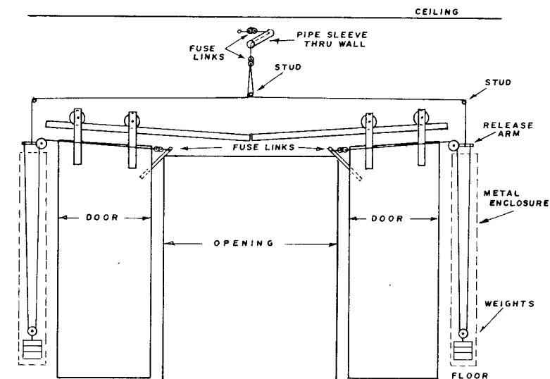
Figure A-38. Closing devices for center parting horizontally sliding doors (inclined track.)
