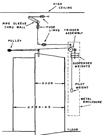
Figure A-30. Closing devices for single swinging door.
