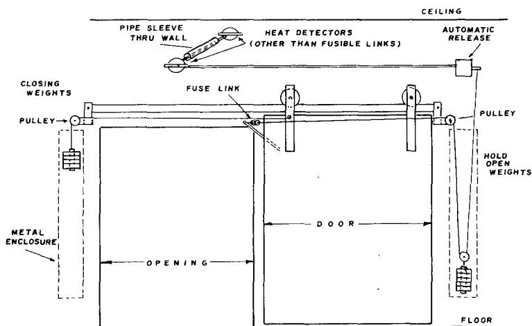
Figure A-36. Closing devices for single sliding door (level track.)
