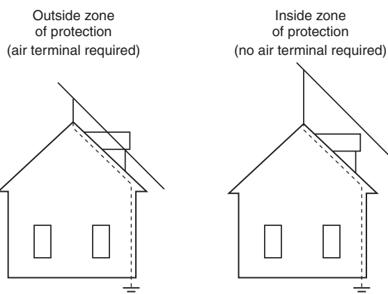
FIGURE A.4.8.4 Dormer Protection.
