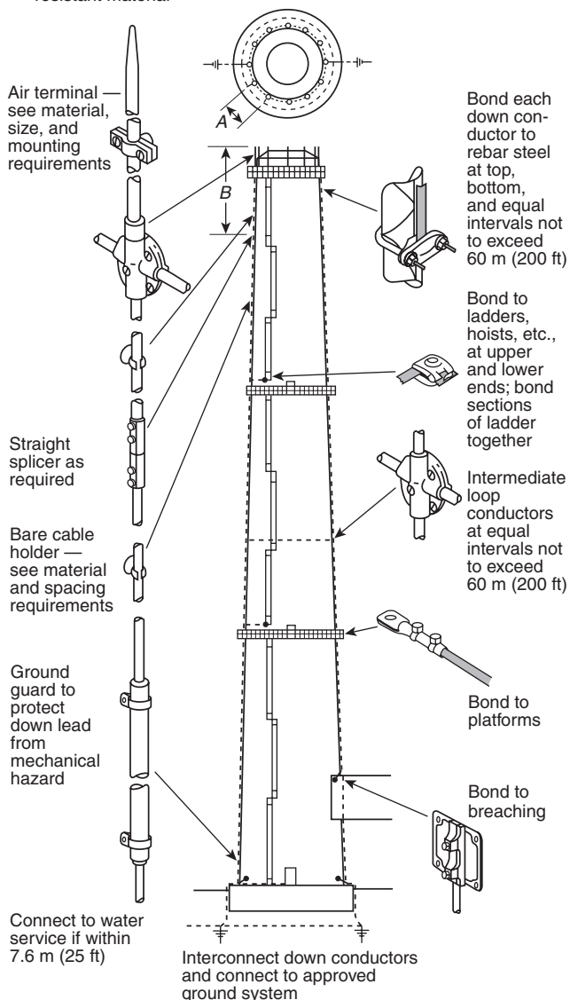
FIGURE 6.1 Heavy-Duty Stack.
