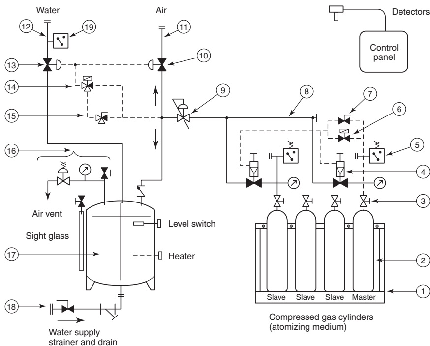
FIGURE A.11.1.6(b) Schematic Representation of a High Pressure, Gas-Driven System with Multiple Accumulator Units for Extended Duration. [Typical]
