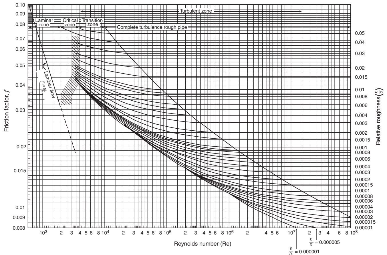
FIGURE 9.2.2 Moody Diagram.
