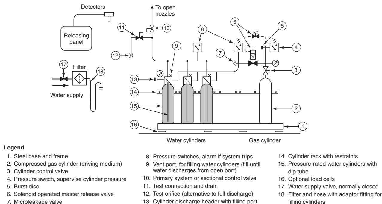
FIGURE A.11.1.6(a) Schematic Representation of a High Pressure, Gas-Driven System with Stored Water (Pre-Engineered System). [Typical]
