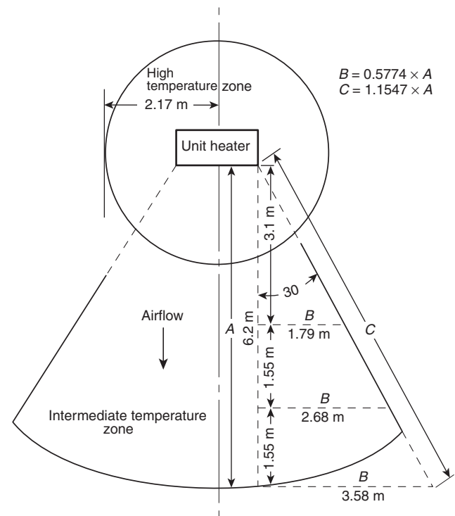
FIGURE 7.2.10.2 High Temperature and Intermediate Temperature Zones at Unit Heaters.
