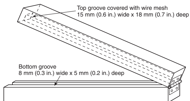
FIGURE C.1.1 Mounting Jig for Test Method 1 Specimens.
