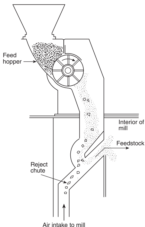
Figure A-4-1.1(a) Pneumatic separator.
