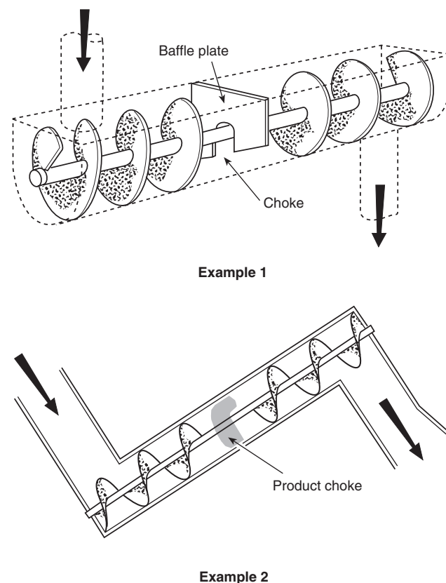
Figure A-3-9.2(a) Screw conveyor chokes.
