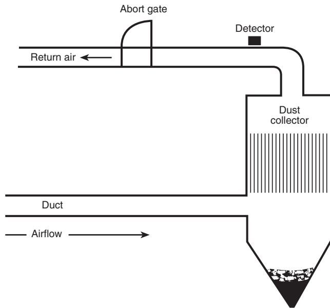
Figure B-1.2 Spark detectors and abort gate.
