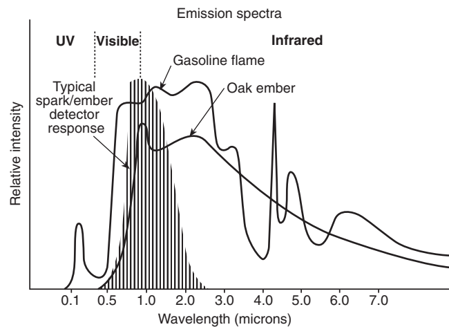
Figure B-1.6 The emissions of an oak ember and gasoline flame compared to the spectral sensitivity of a spark/ember detector.
