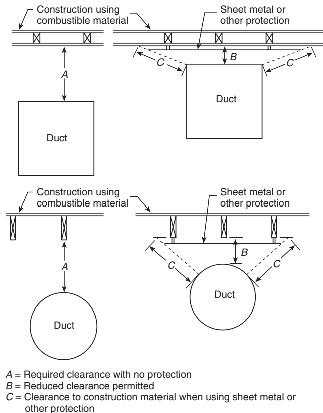
Figure 2-6.4 Extent of protection required to reduce clearances from ducts
