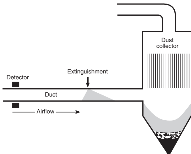
Figure B-1.3 The typical spark detection and extinguishment system.
