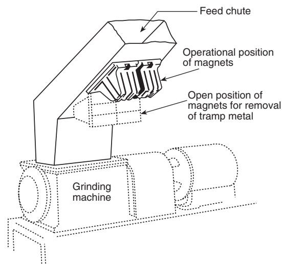
Figure A-4-1.1(b) Magnetic separator.
