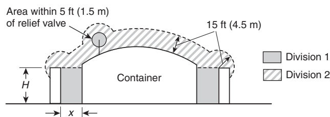
FIGURE A.10.6.2(b) Dike Height Greater than Distance from Container to Dike ( H > x ).
