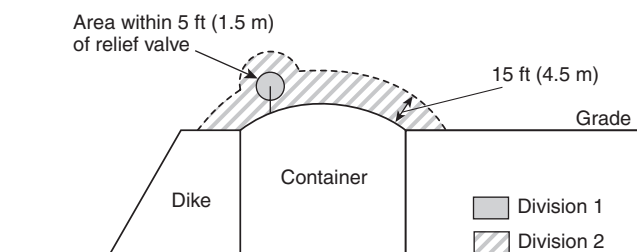
FIGURE A.10.6.2(c) Container with Liquid Level Below Grade or Below Top of Dike.
