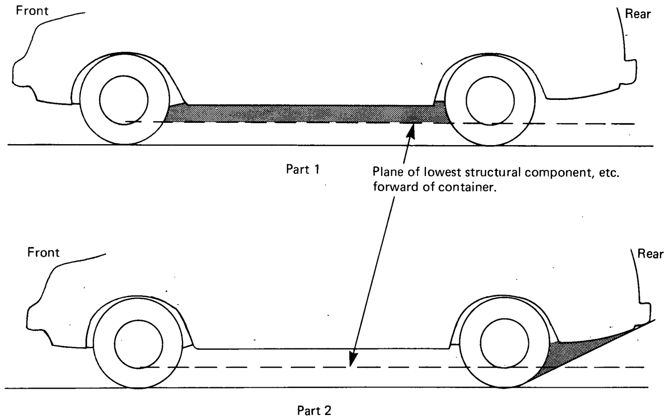
Figure 3-6.2.6(e) Container Installation Clearances
