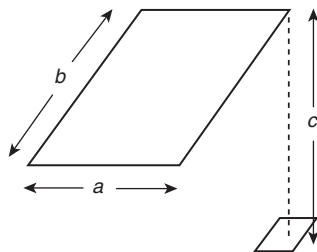
FIGURE 10.3.6(b) Configuration Factor for One Quadrant of the Hot Gas Layer to a Target Not Facing the Hot Layer.
