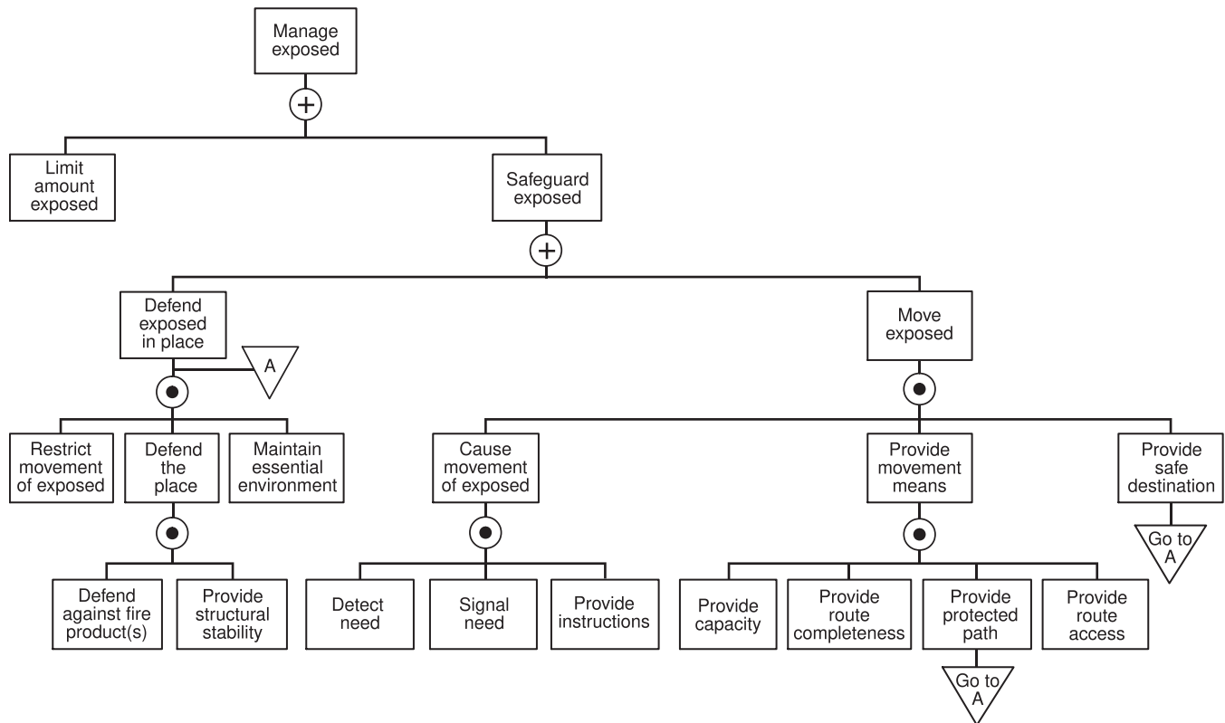
FIGURE 4.5.2.1 “Manage Exposed” Branch of Fire Safety Concepts Tree.
