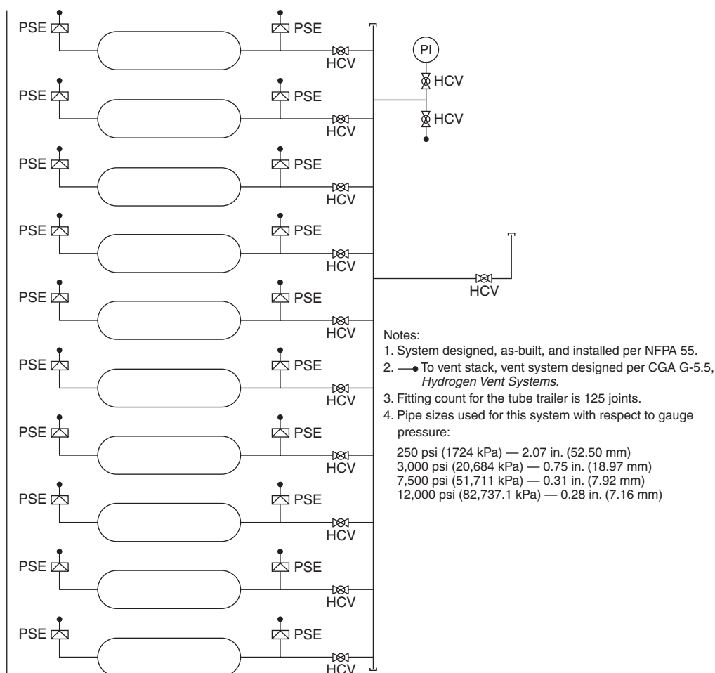
FIGURE A.3.3.57.1(b) Typical Tube Trailer. [55:Figure A.3.3.12(b)]
