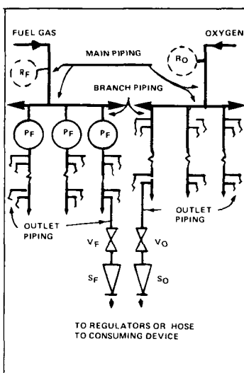
FIGURE 2 OPTION 2 P F IN BRANCH
