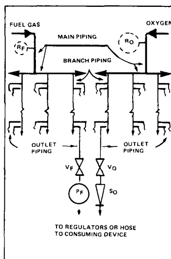
FIGURE 3 OPTION 3 P F IN OUTLET PIPING
