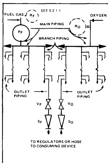
FIGURE 1 OPTION 1 P F IN MAIN
