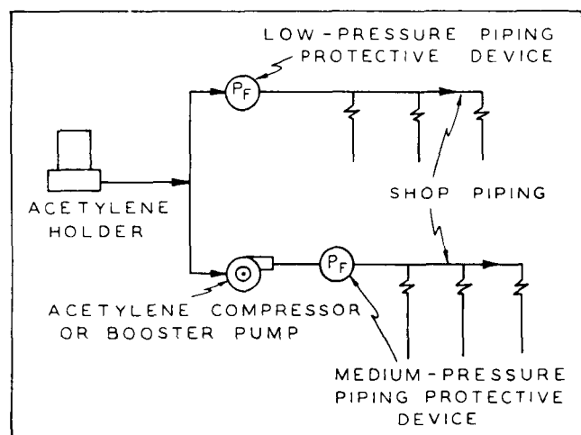
Figure 4 Protective Devices for Gas Holders, Compressors, and Booster Pumps.
