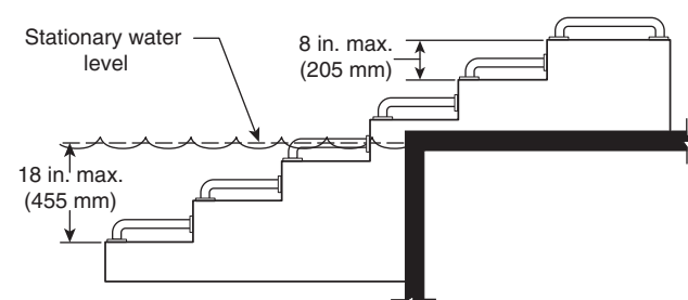
FIGURE 12.45.15.5.4 Transfer Steps. [ADA/ABA-AG: Figure 1009.5.4]
