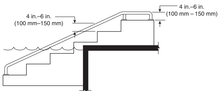
(b) Continuous Grab Bars
