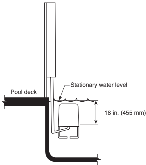
FIGURE 12.45.15.2.8 Pool Lift Submerged Depth. [ADA/ABA-AG: Figure 1009.2.8]
