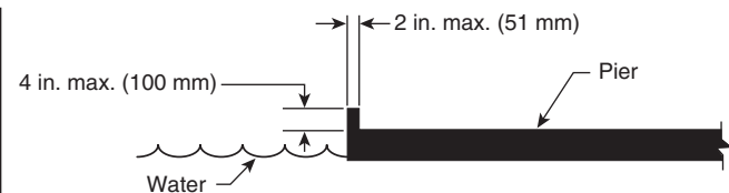
FIGURE 12.45.9.3.1(c) Edge Protection at Boat Slips. [ADA/ABA-AG: Figure 1003.3.1, Exception 2]
