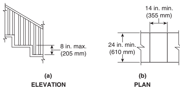
FIGURE 12.45.14.3.2 Transfer Steps. [ADA/ABA-AG: Figure 1008.3.2]
