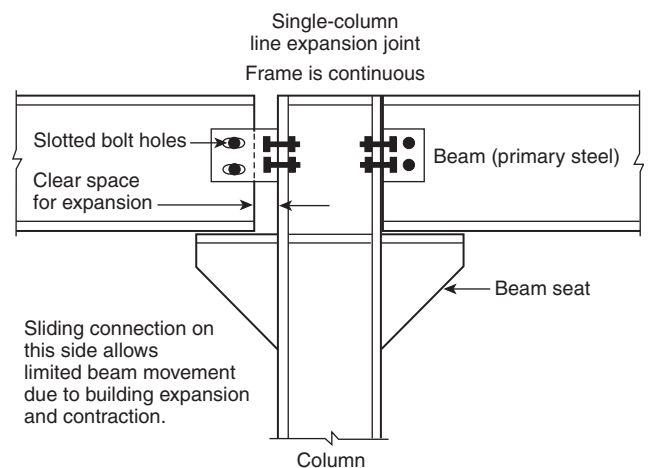
FIGURE A.8.3.2.4(e) Single-Column Line Expansion Joint Frame Is Continuous. [221:Figure A.5.4(e)]
