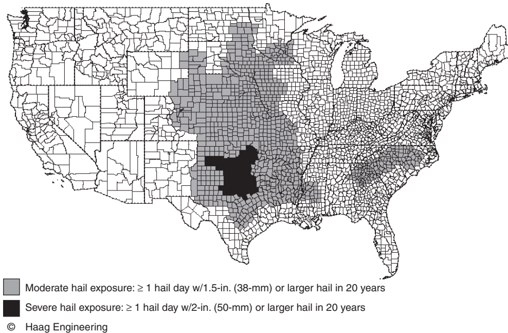
FIGURE 38.5.1 Hail Exposure Map.
