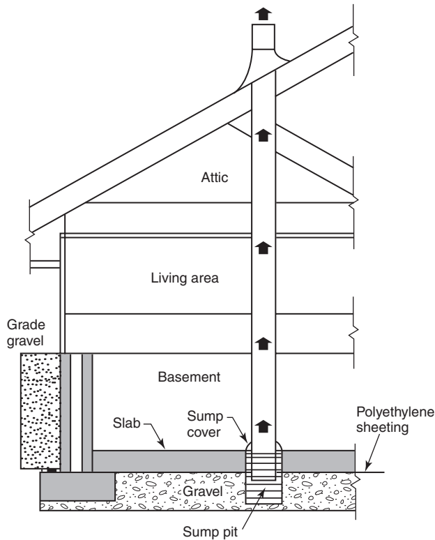
FIGURE 49.2.5.3.3.4 Passive Radon System Vented Through Sump.
