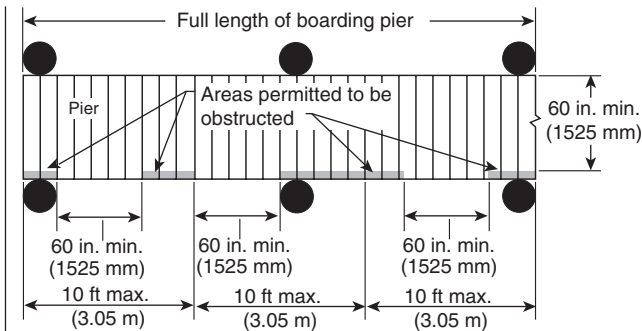
FIGURE 12.45.9.3.2(a) Boarding Pier Clearance. [ADA/ABA-AG: Figure 1003.3.2]
