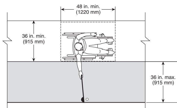
FIGURE 12.45.13.3.2 Golf Club Reach Range Area. [ADA/ABA-AG: Figure 1007.3.2]
