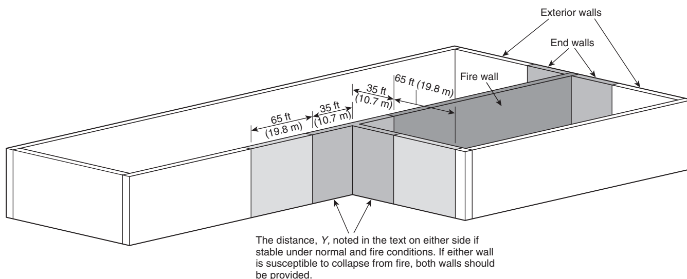
FIGURE 8.3.2.16.3.1 Angle Wall Exposure Protection. [221: Figure 5.16.3.1]
