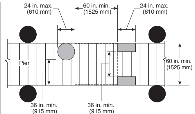
FIGURE 12.45.9.3.1(b) Clear Pier Space Reduction at Boat Slips. [ADA/ABA-AG: Figure 1003.3.1, Exception 1]
