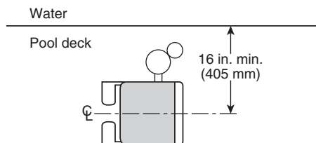
FIGURE 12.45.15.2 Pool Lift Seat Location. [ADA/ABA-AG: Figure 1009.2.2]
