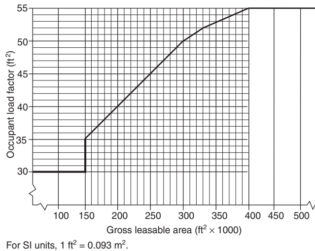
FIGURE 11.3.1.2 Mall Building Occupant Load Factors.
