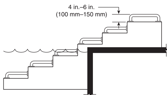
(a) Individual Grab Bars
