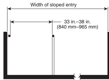
FIGURE 12.45.15.3.3 Handrails for Sloped Entry. [ADA/ABA-AG: Figure 1009.3.3]
