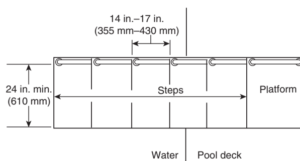
FIGURE 12.45.15.5.6 Size of Transfer Steps. [ADA/ABA-AG: Figure 1009.5.6]
