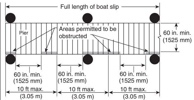
FIGURE 12.45.9.3.1(a) Boat Slip Clearance. [ADA/ABA-AG: Figure 1003.3.1]
