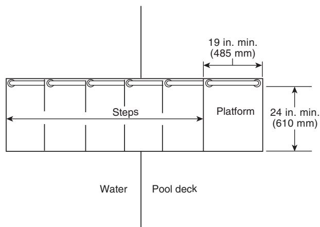
FIGURE 12.45.15.5.1 Size of Transfer Platform. [ADA/ABA-AG: Figure 1009.5.1]
