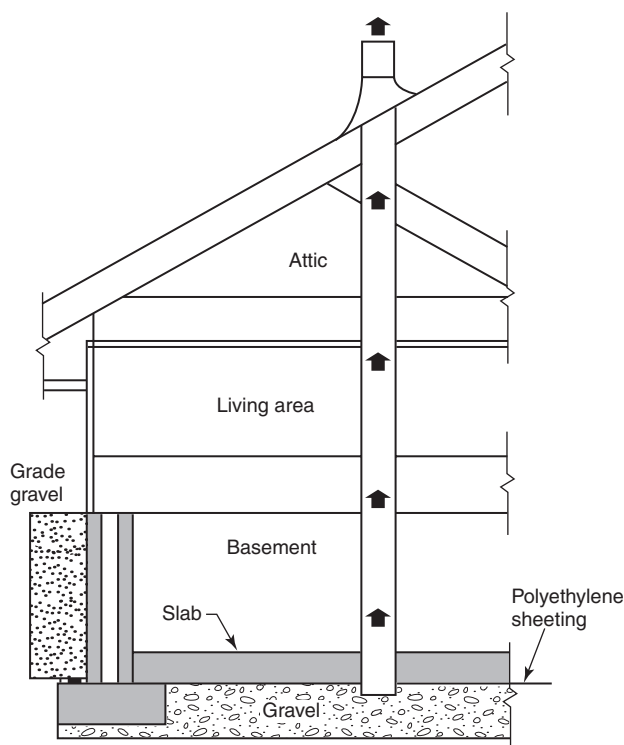
FIGURE 49.2.5.3.5 Passive Sub-Slab Depressurization Radon System.
