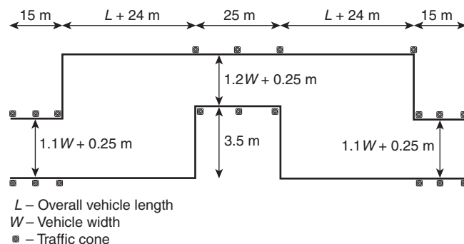
FIGURE 6.3.2.5.3 Lane Change Test Course.
