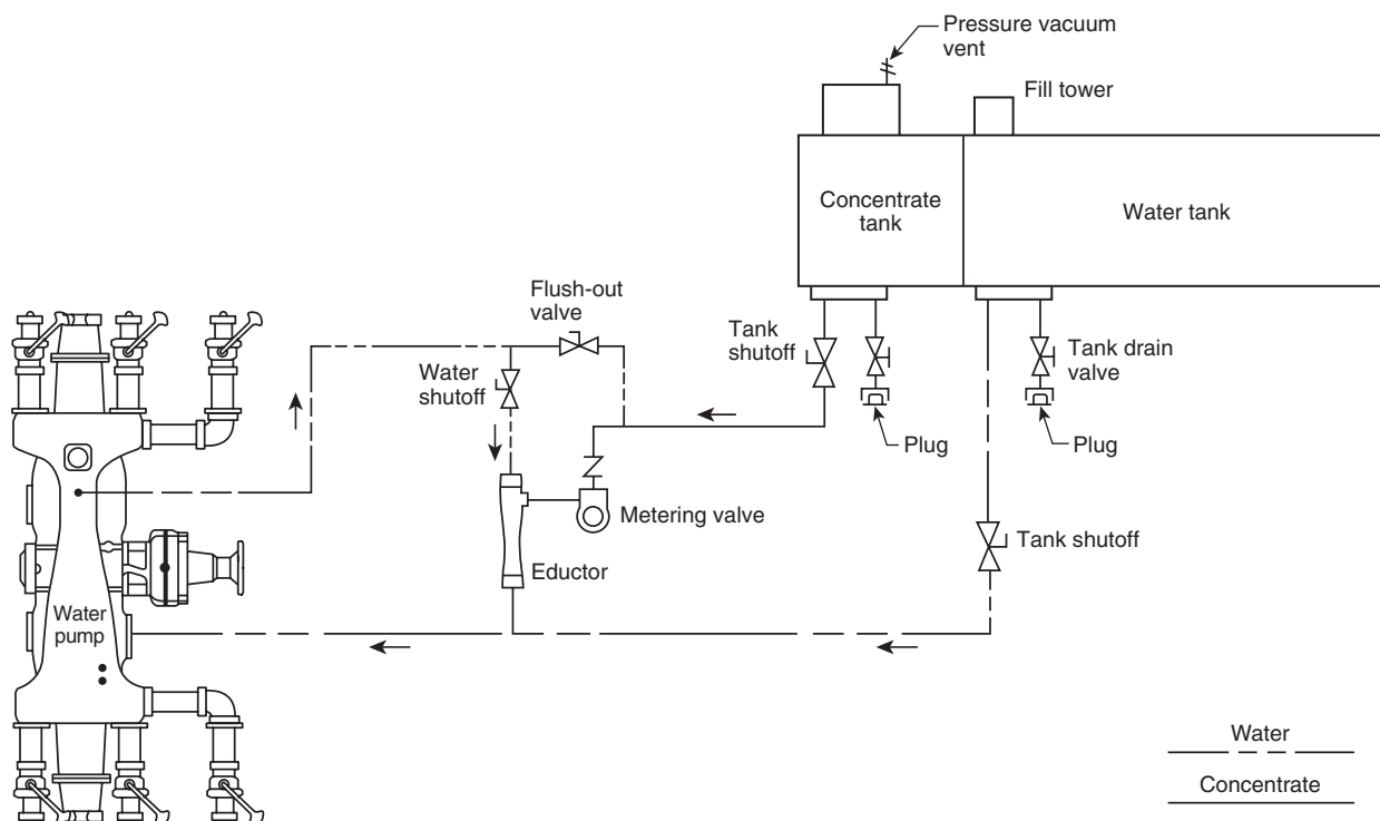
FIGURE A.4.17(a) Manual Variable Metering, Around-the-Pump Proportioning System.
