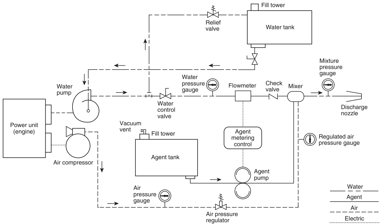
FIGURE A.4.17(h) Compressed Air-Foam System.
