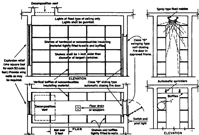
Figure 4-3 Standard Film Vault (for other than archival film).
