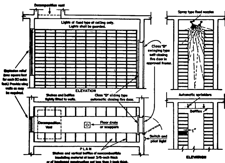
Figure 4-5 Archival Vault.
