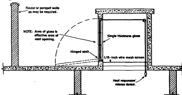
Figure 4-3.3 Decomposition Vent.
