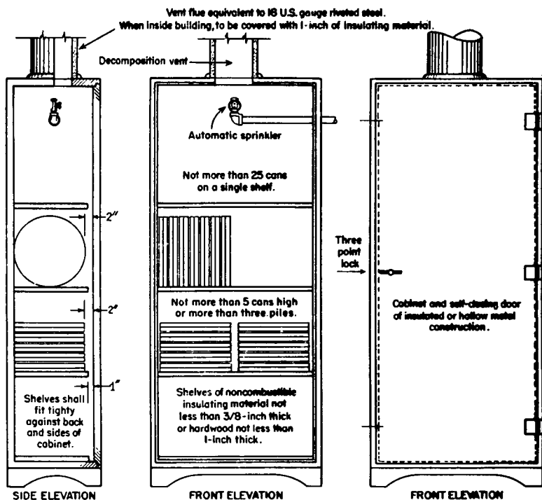
Figure 4-2 Standard Film Cabinet (for other than archival film).
