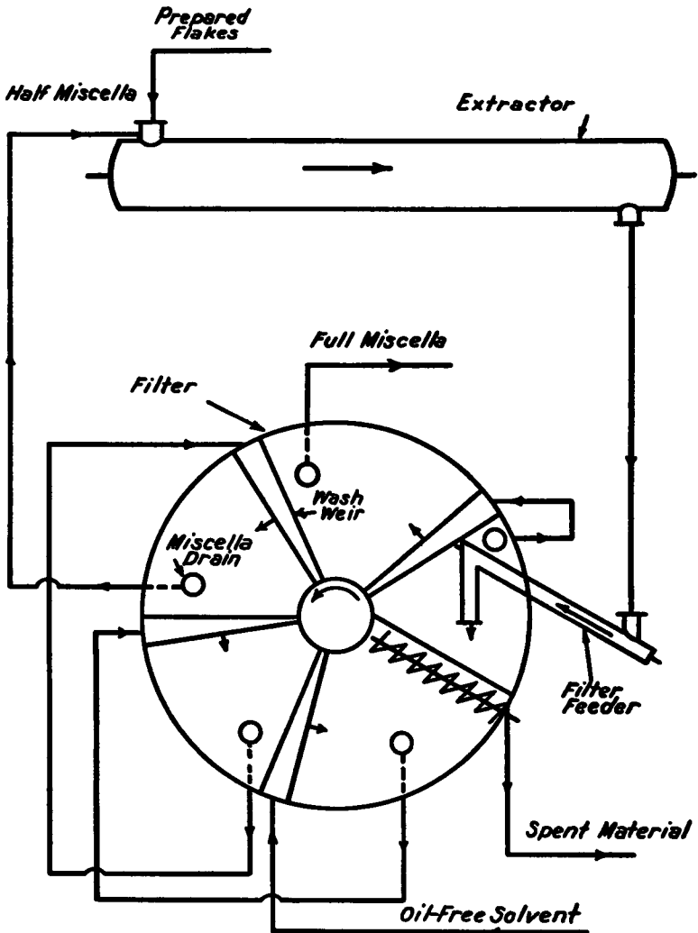
Figure A-7 Filtration-type Extractor.
