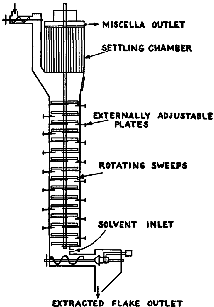
Figure A-6 Vertical Total Immersion Extractor.
